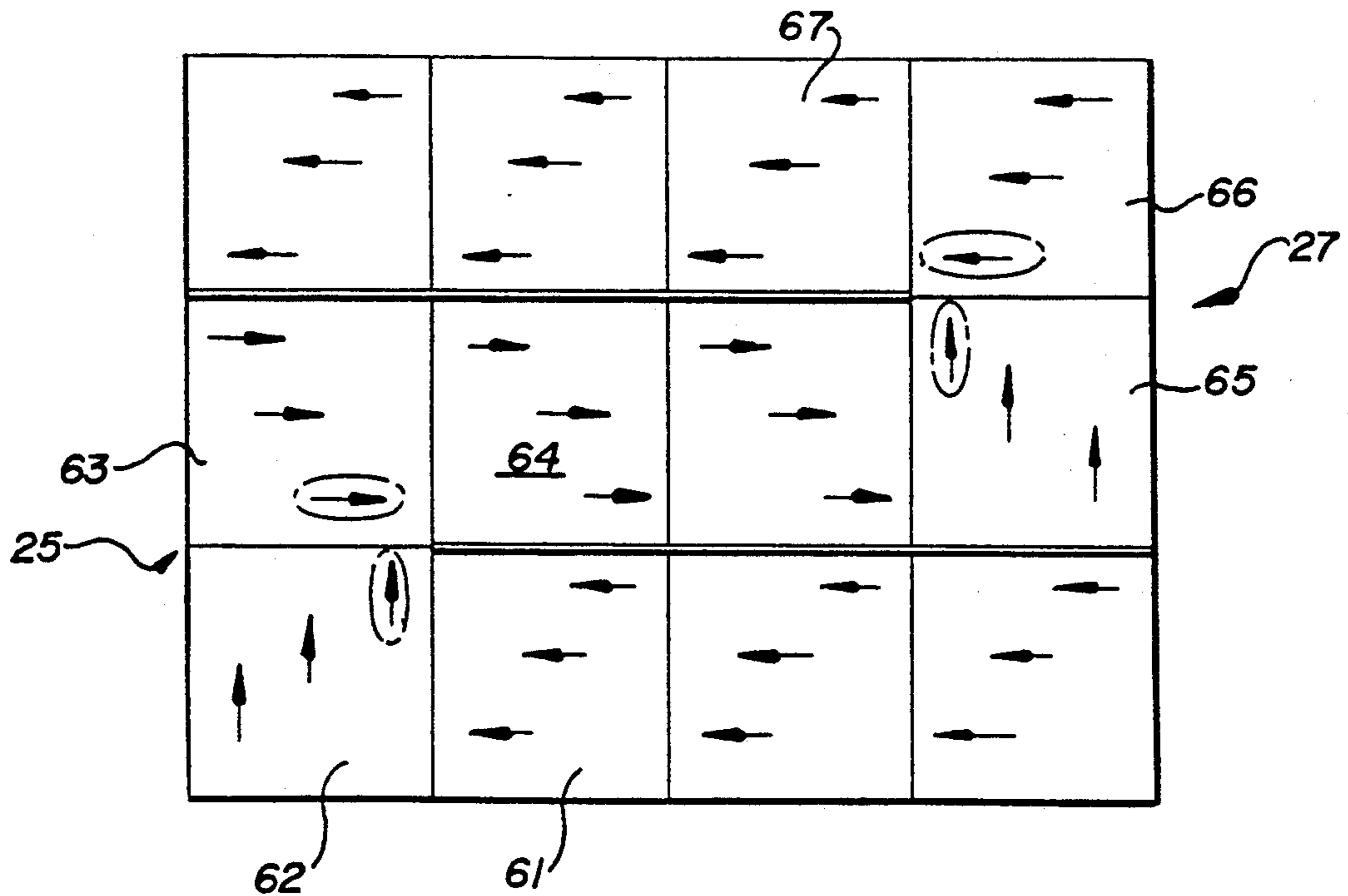
FIG. 6 PRIOR ART
