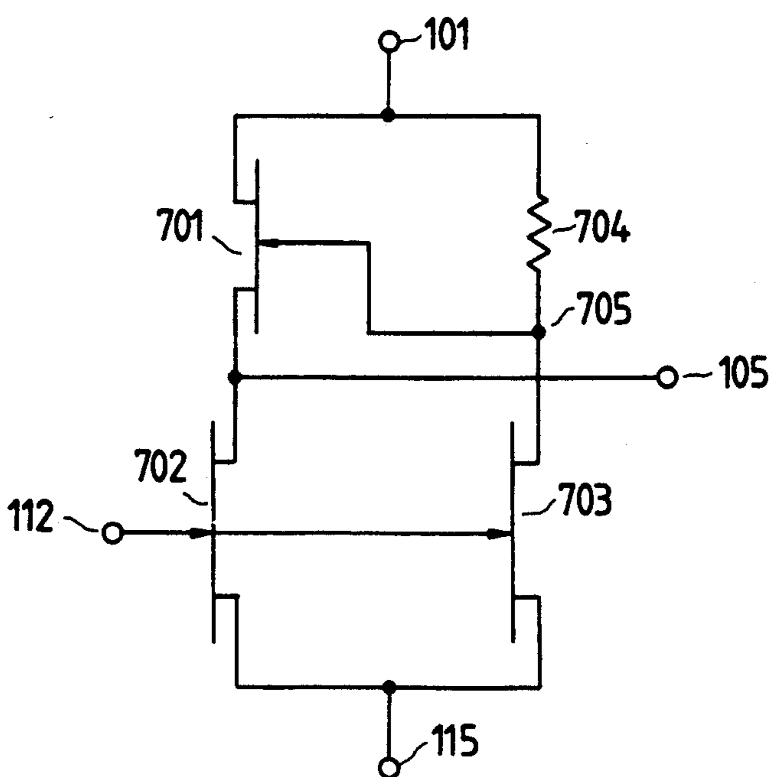
FIG. 7 PRIOR ART
