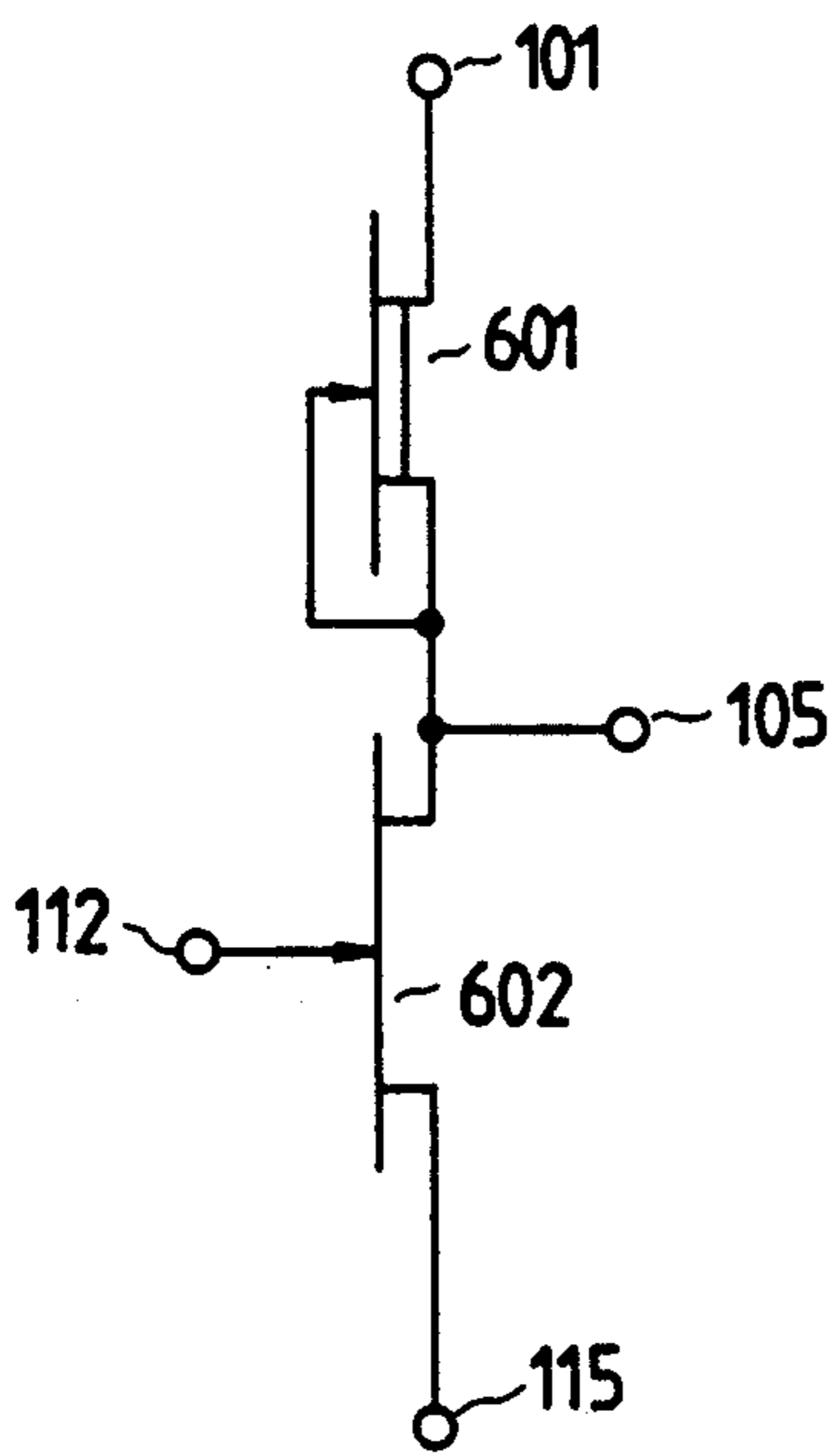
FIG. 6 PRIOR ART
