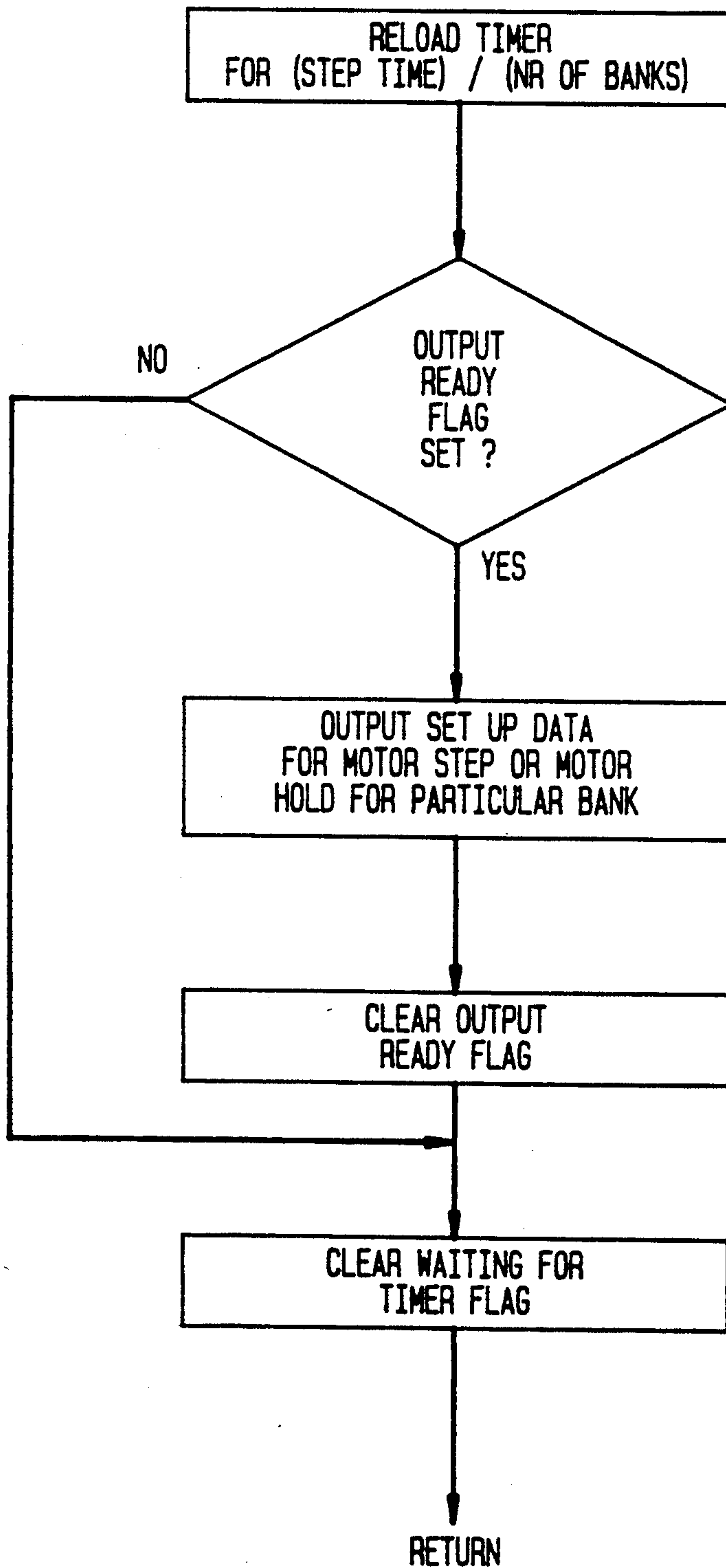
FIG. 19F TIMER INTERRUPT ROUTINE
