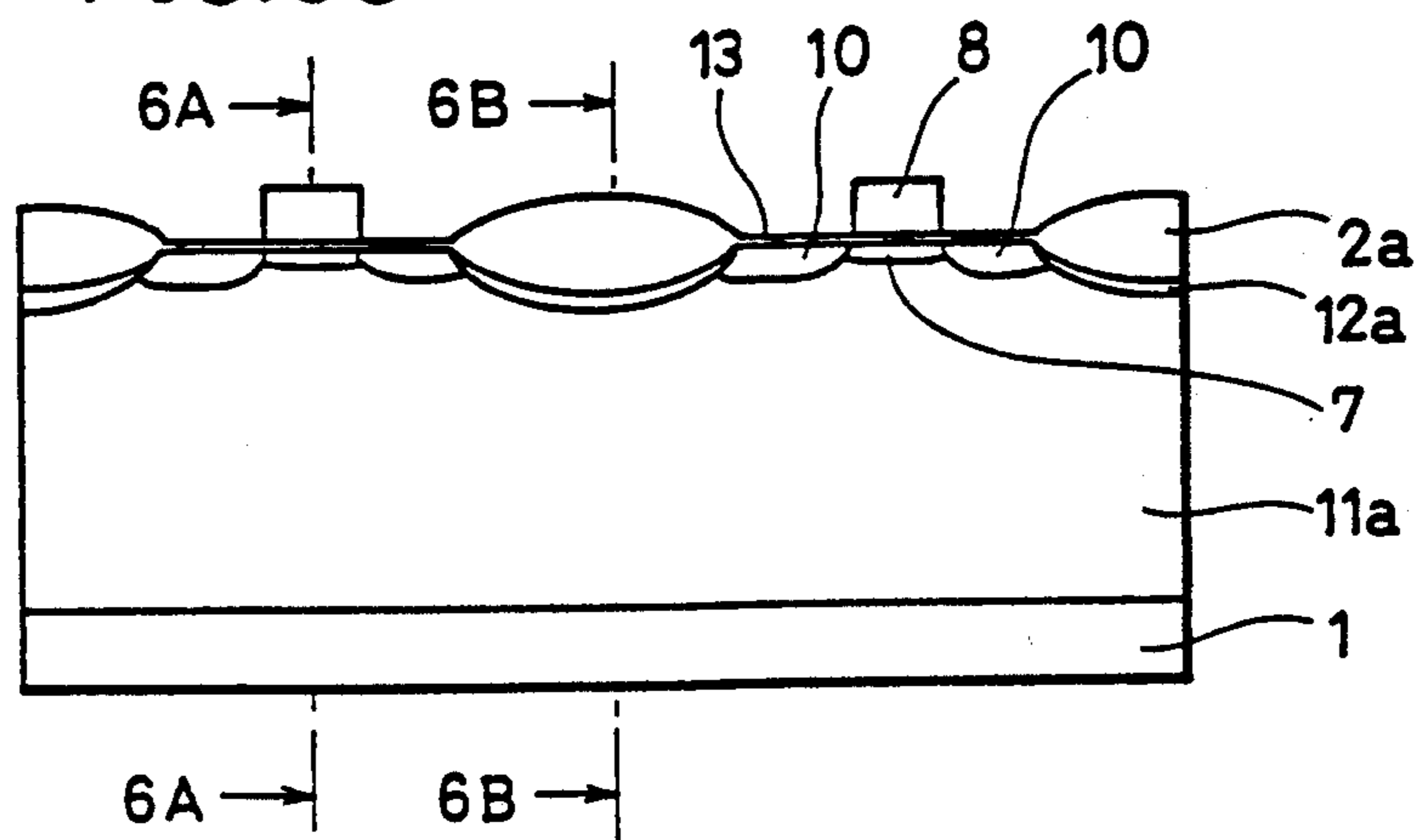
FIG.5G PRIOR ART
