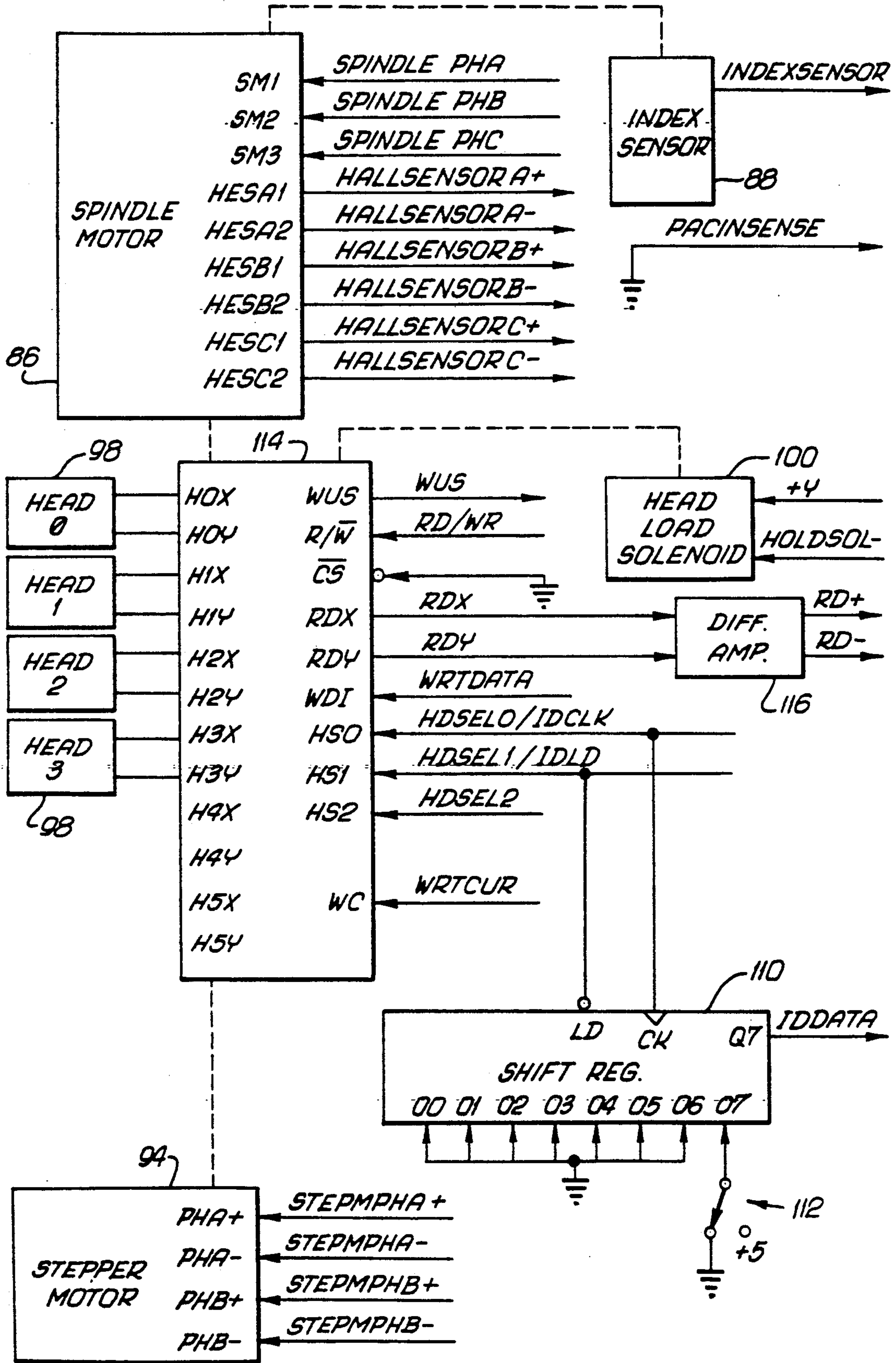
FIG. 4 DISK DRIVE -80-
