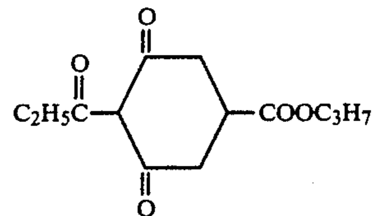
Compound 4: Calcium 3,5-dioxo-4-propionylcyclohexane carboxylate
