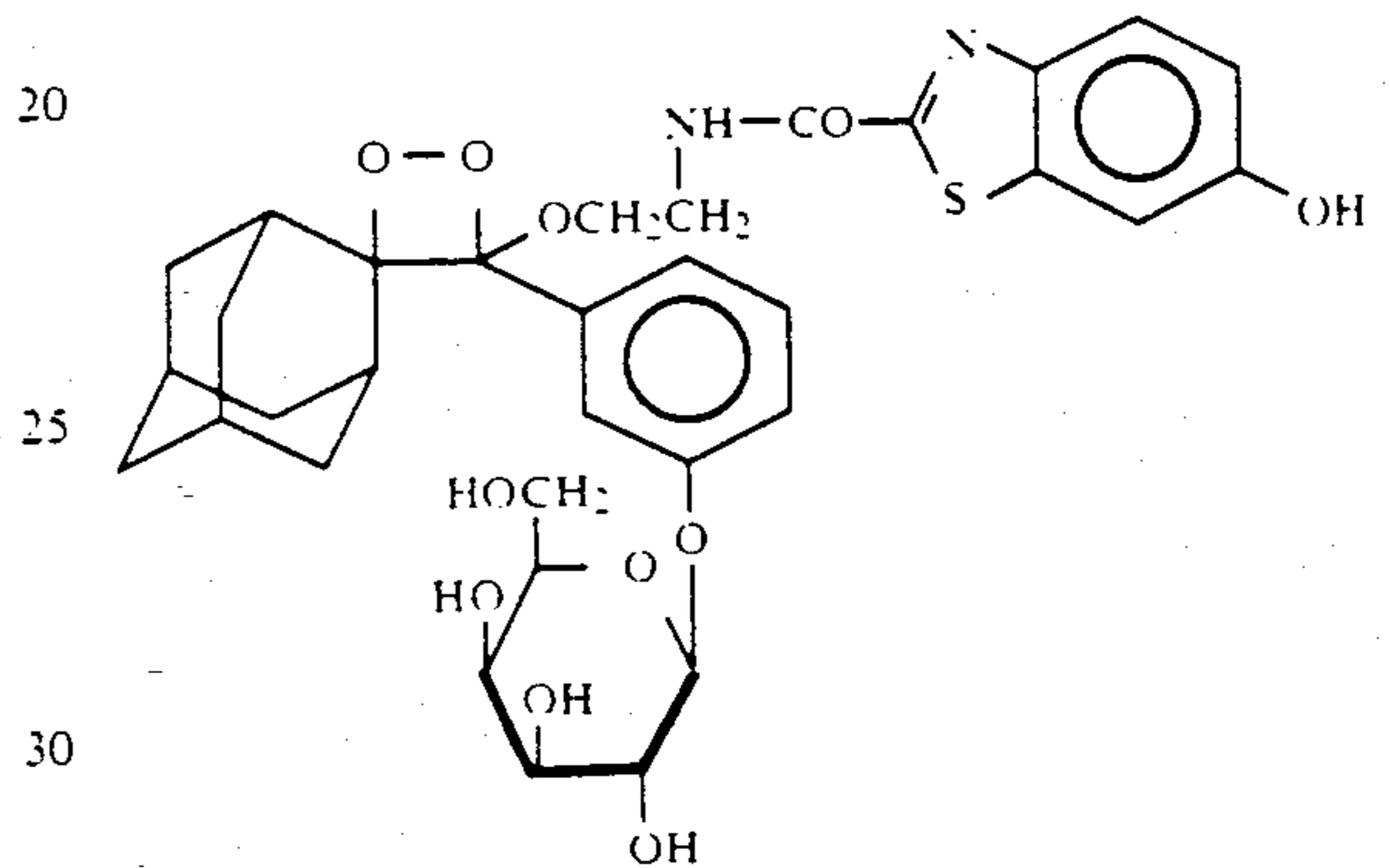
4-(3-Phosphatephenyl)-4-(2-(O-fluorescein)ethoxy)spiro[1.2-dioxetane-3,2'-adamantane] (10) and 4-(2-(N-(6-hydroxybenzothiazole-2-carbonyl)amino)ethoxy)-4-(3-phosphatephenyl)spiro[1.2-dioxetane-3,2'-adamantane] (12) are prepared using the photooxygenation procedures described above from alkenes 9 and 11, respectively. 35 40
