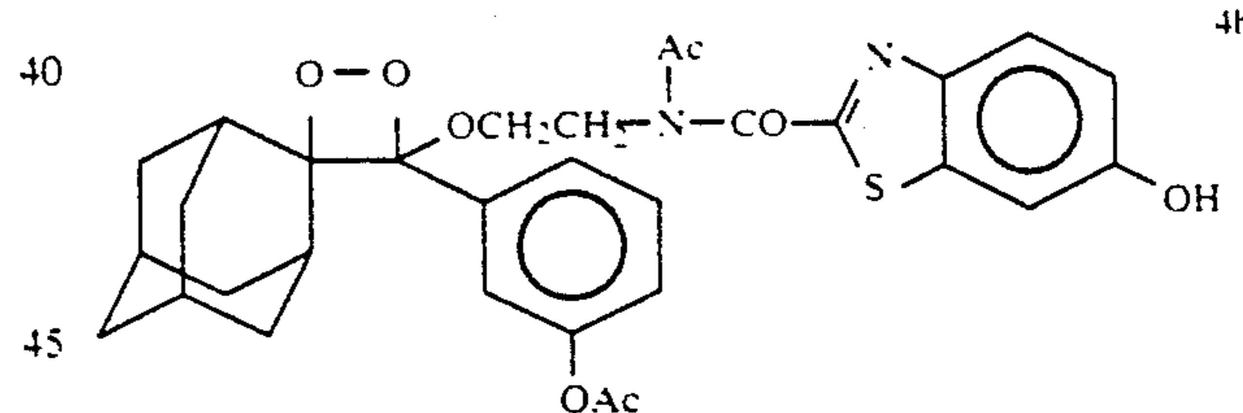
4-(3-Acetoxyphenyl)-4-(2-(O-fluorescein)ethoxy)spiro[1,2-dioxetane-3,2'-adamantane] (6)
