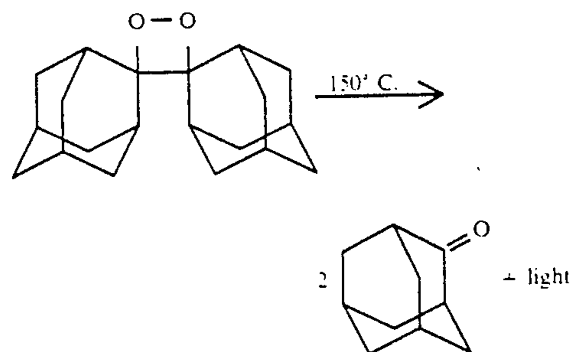
adamantylideneadamantane
