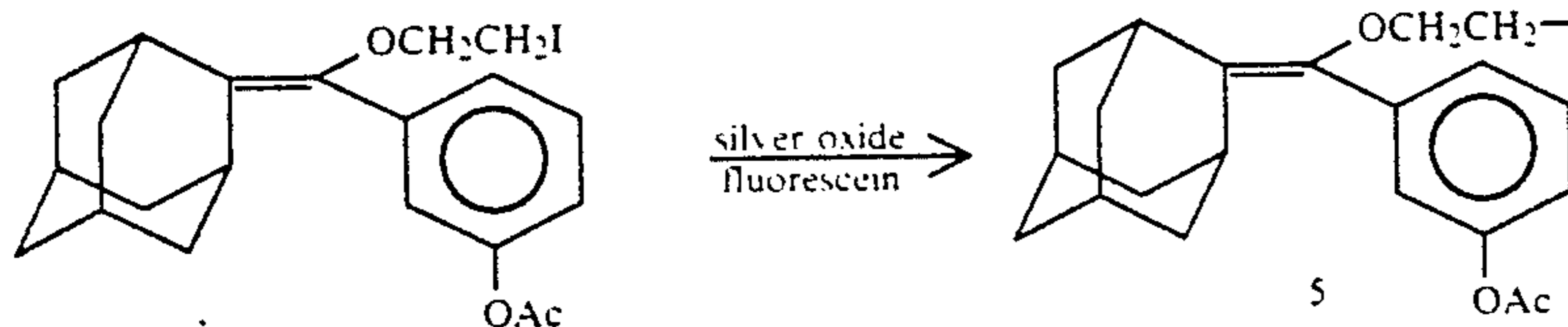
[(2-Aminoethoxy)(3- \beta -D-galactopyranosylphenyl)methylene]adamantane (5)
