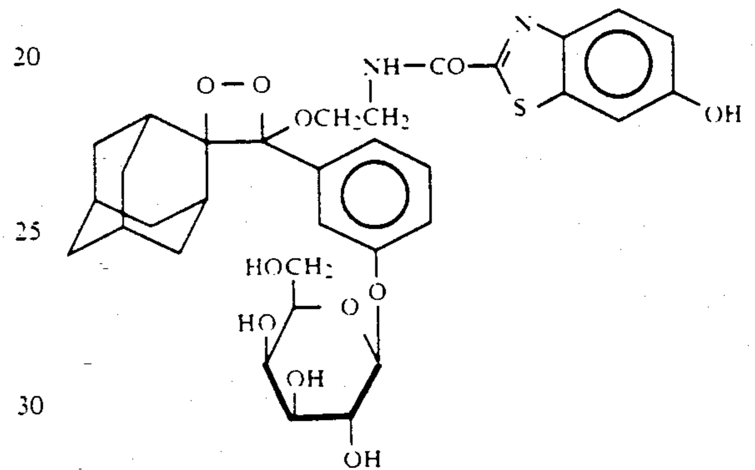
4-(3-Phosphatephenyl)-4-(2-(O-fluorescein)ethoxy)spiro[1.2-dioxetane-3,2'-adamantane] (10) and 4-(2-(N-(6-hydroxybenzothiazole-2-carbonyl)amino)ethoxy)-4-(3-phosphatephenyl)spiro[1.2-dioxetane-3,2'-adamantane] (12) are prepared using the photooxygenation procedures described above from alkenes 9 and 11, respectively. 35 40
