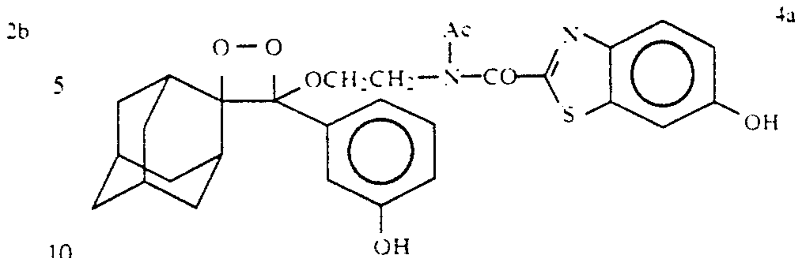
4-(3-Acetoxyphenyl)-4-(2-(N-acetyl-N-(6-hydroxybenzothiazole-2-carbonyl)amino)ethoxy)spiro[1,2-dioxetane-3,2'-adamantane] (4b)
