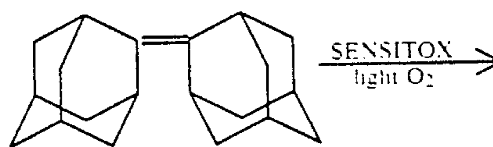
adamantylideneadamantane
