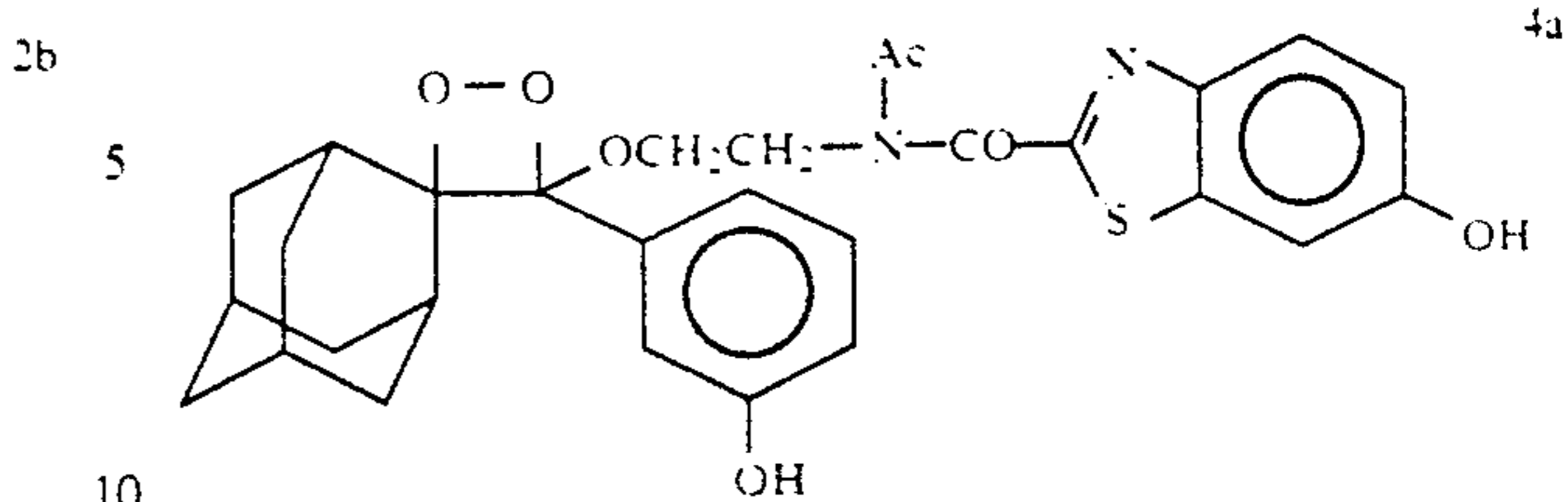
4-(3-Acetoxyphenyl)-4-(2-(N-acetyl-N-(6-hydroxybenzothiazole-2-carbonyl)amino)ethoxy)spiro[1,2-dioxetane-3,2'-adamantane] (4b)
