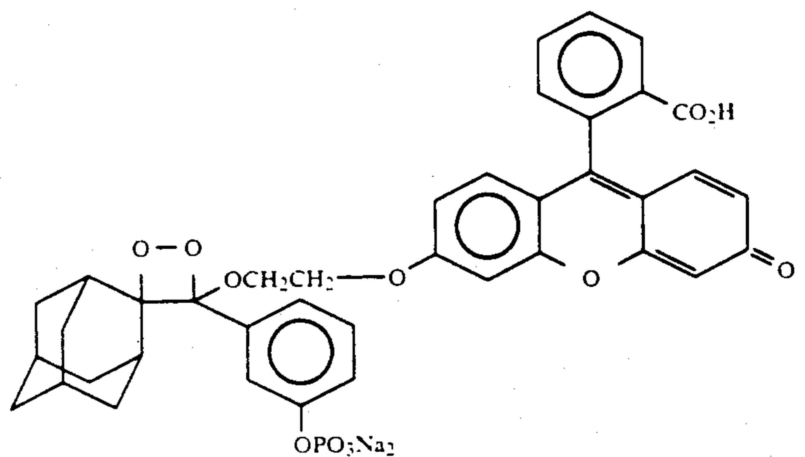
4-(3-Phosphatephenyl)-4-(2-(O-fluorescein)ethoxy)spiro[1.2-dioxetane-3,2'-adamantane] (10) and 4-(2-(N-(6-hydroxybenzothiazole-2-carbonyl)amino)ethoxy)-4-(3-phosphatephenyl)spiro[1.2-dioxetane-3,2'-adamantane] (12) are prepared using the photooxygenation procedures described above from alkenes 9 and 11, respectively. 35 40
