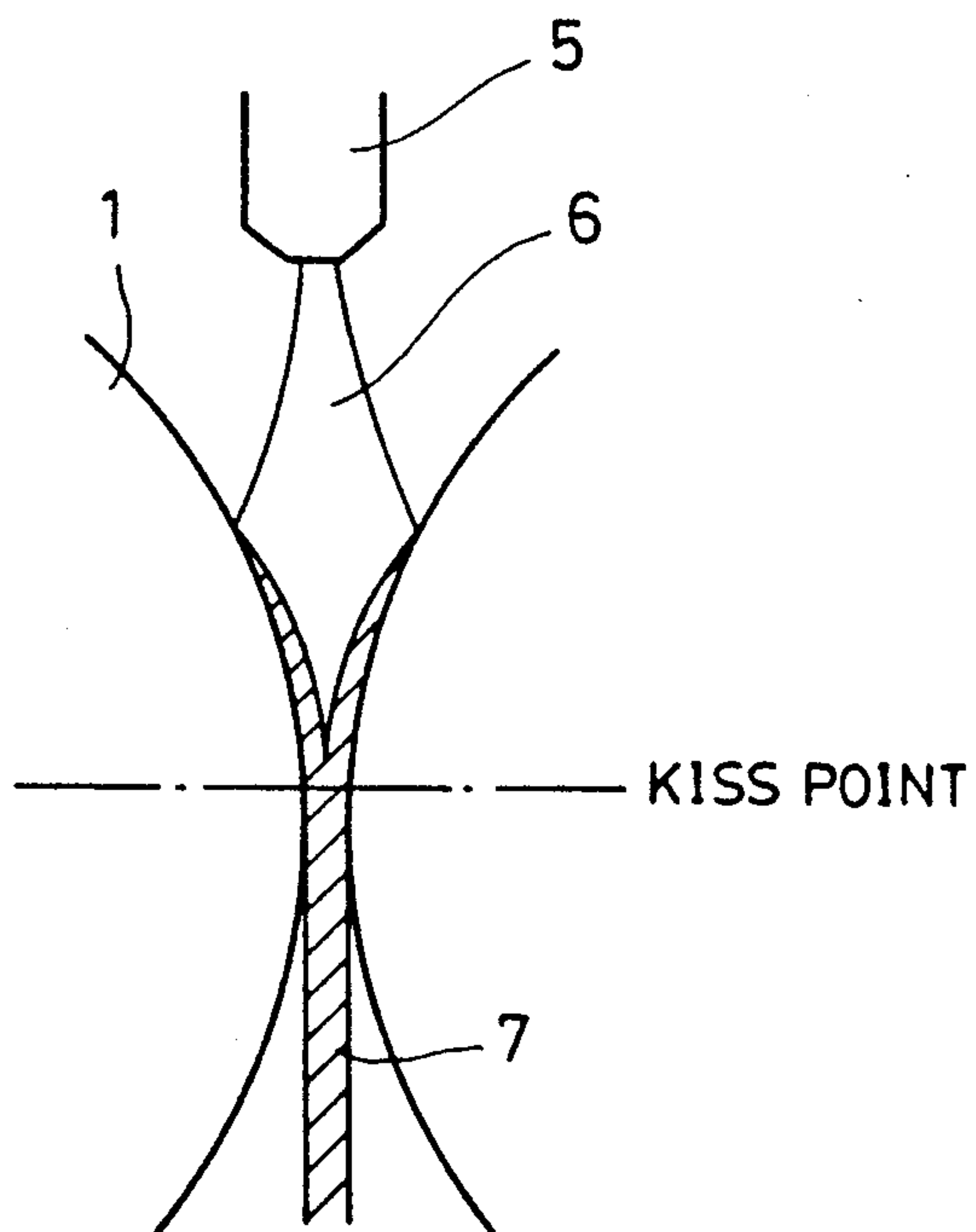
ROLL KISS SOLIDIFICATION COMPLETION TYPE
