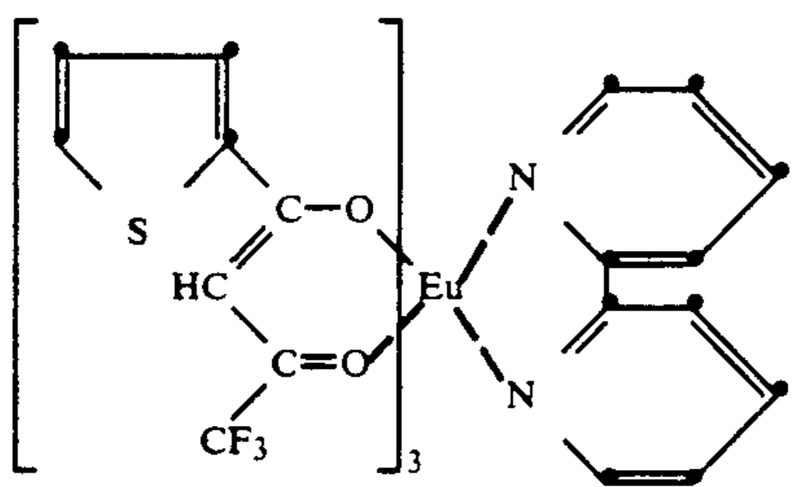
Compound 6
