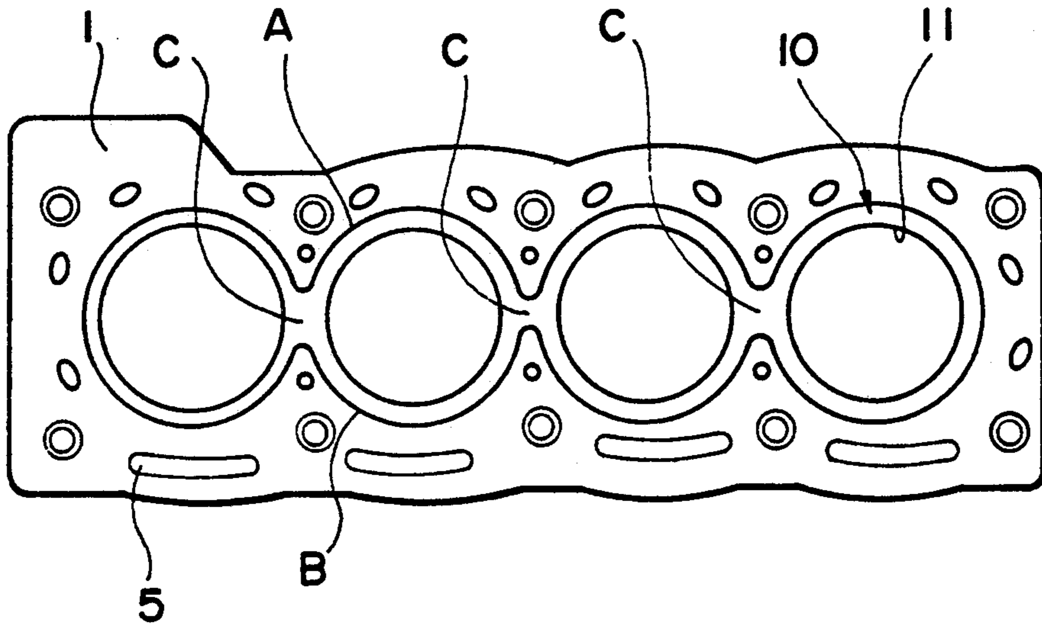
FIG. 5 (PRIOR ART)
