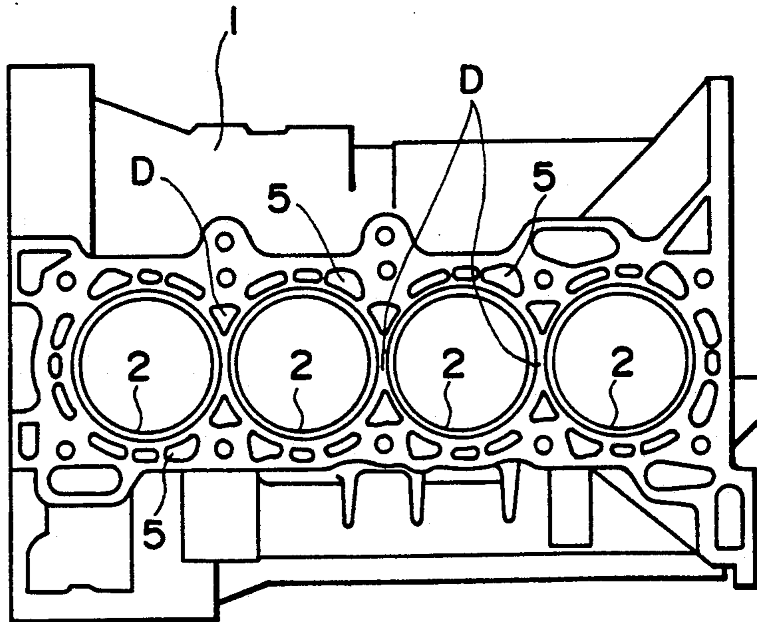
FIG. 6 (PRIOR ART)
