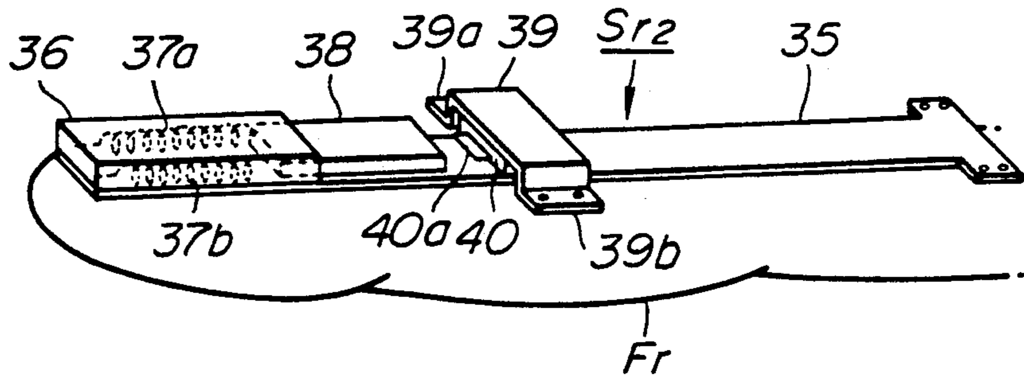
FIG. 5 (PRIOR ART)
