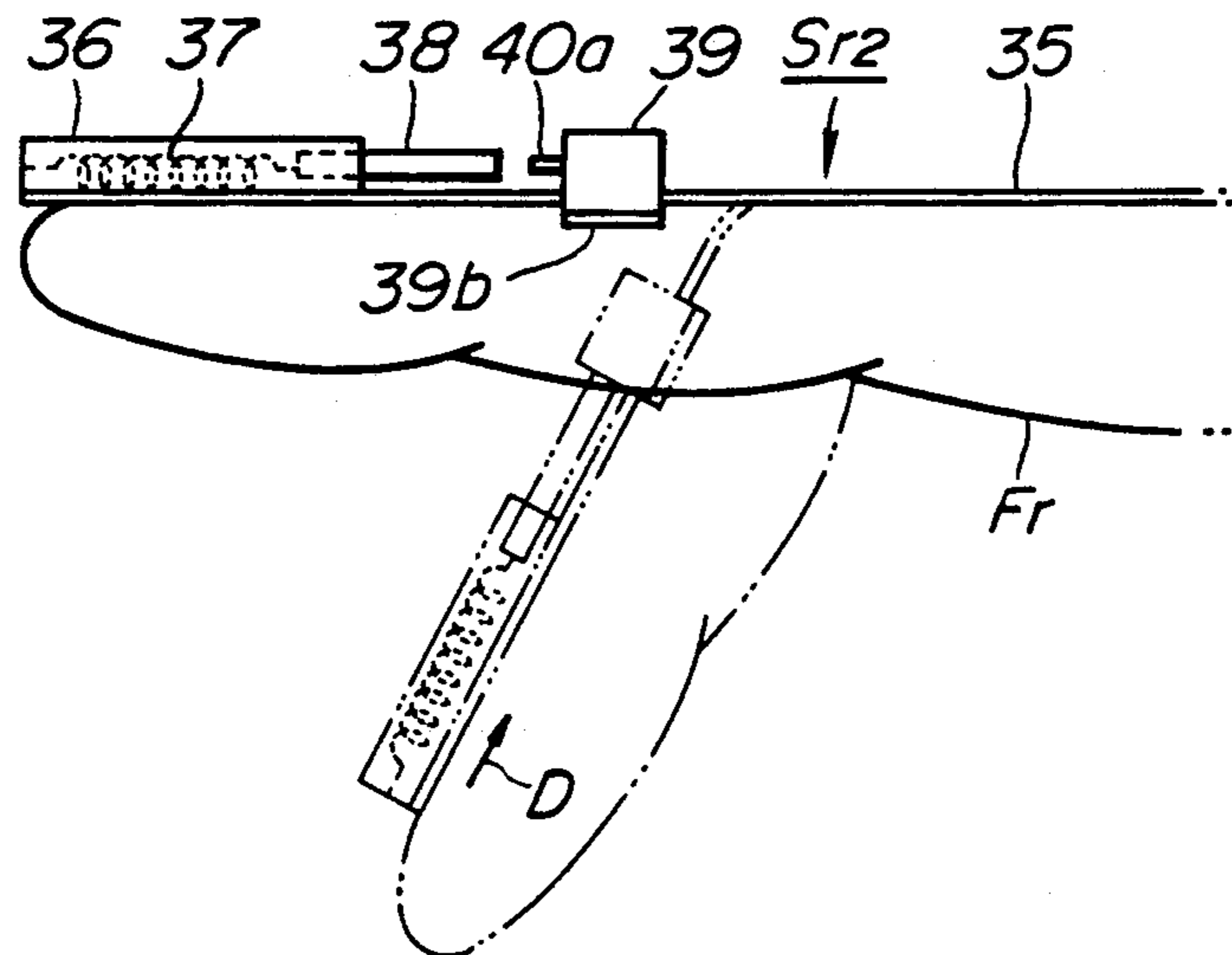
FIG. 6 (PRIOR ART)
