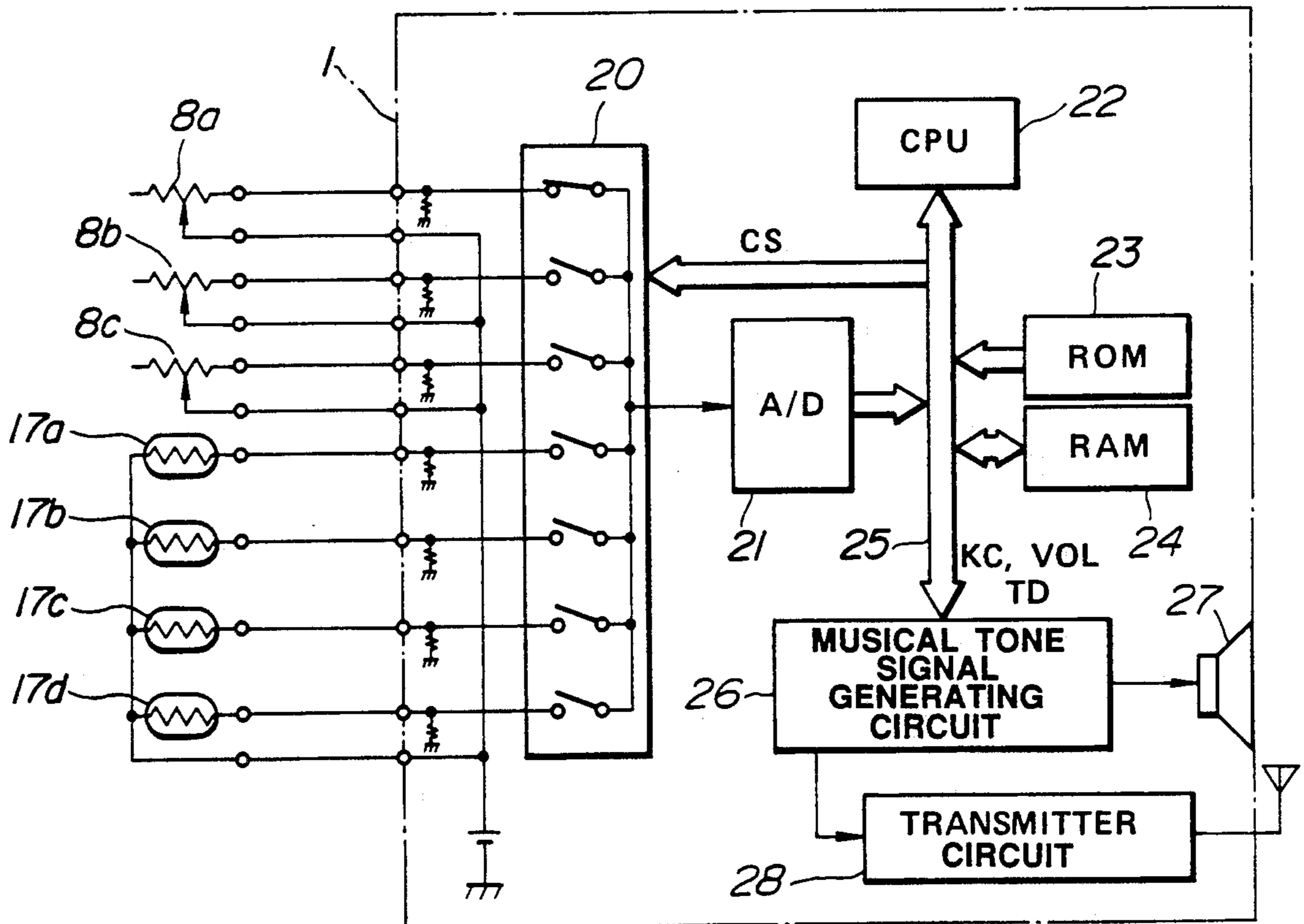
FIG. 2 (PRIOR ART)
