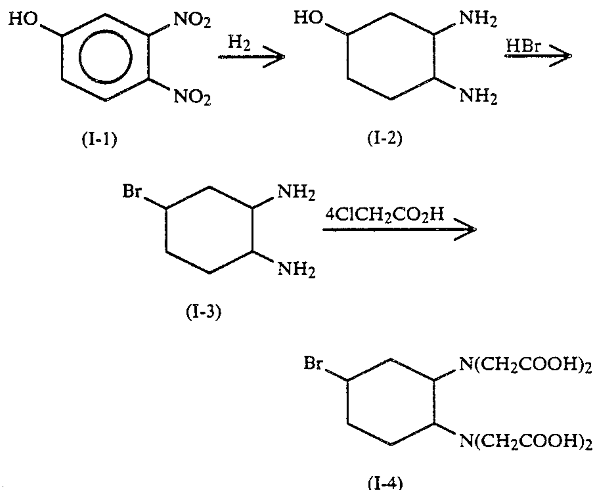
Scheme I: Preparation of Bromo-DCTA
