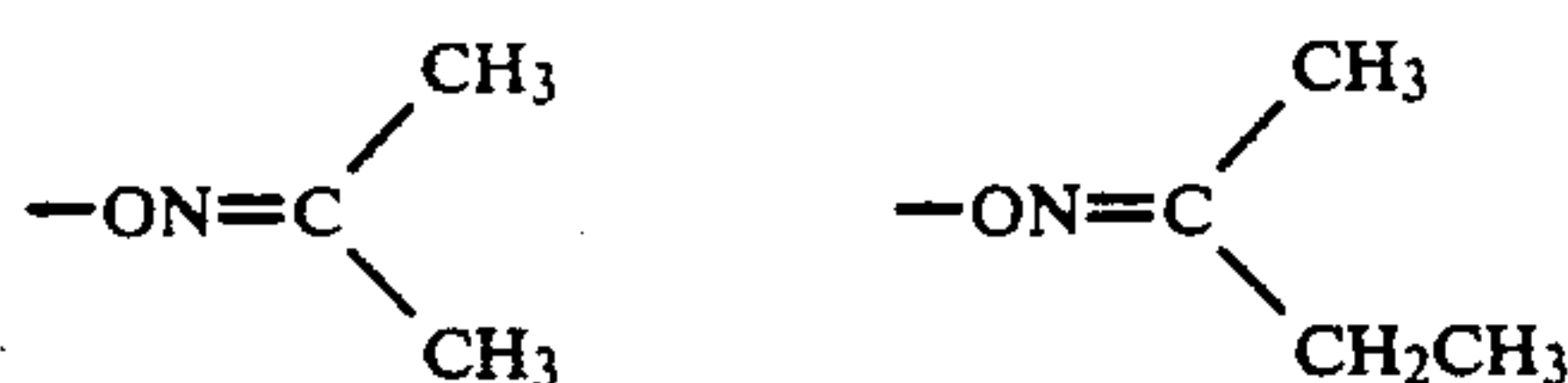
Acetone Oxime
