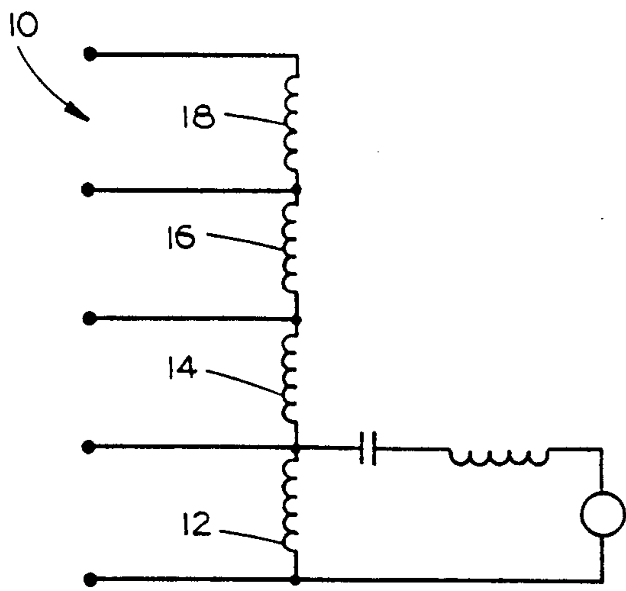
FIG. 1 (PRIOR ART)
