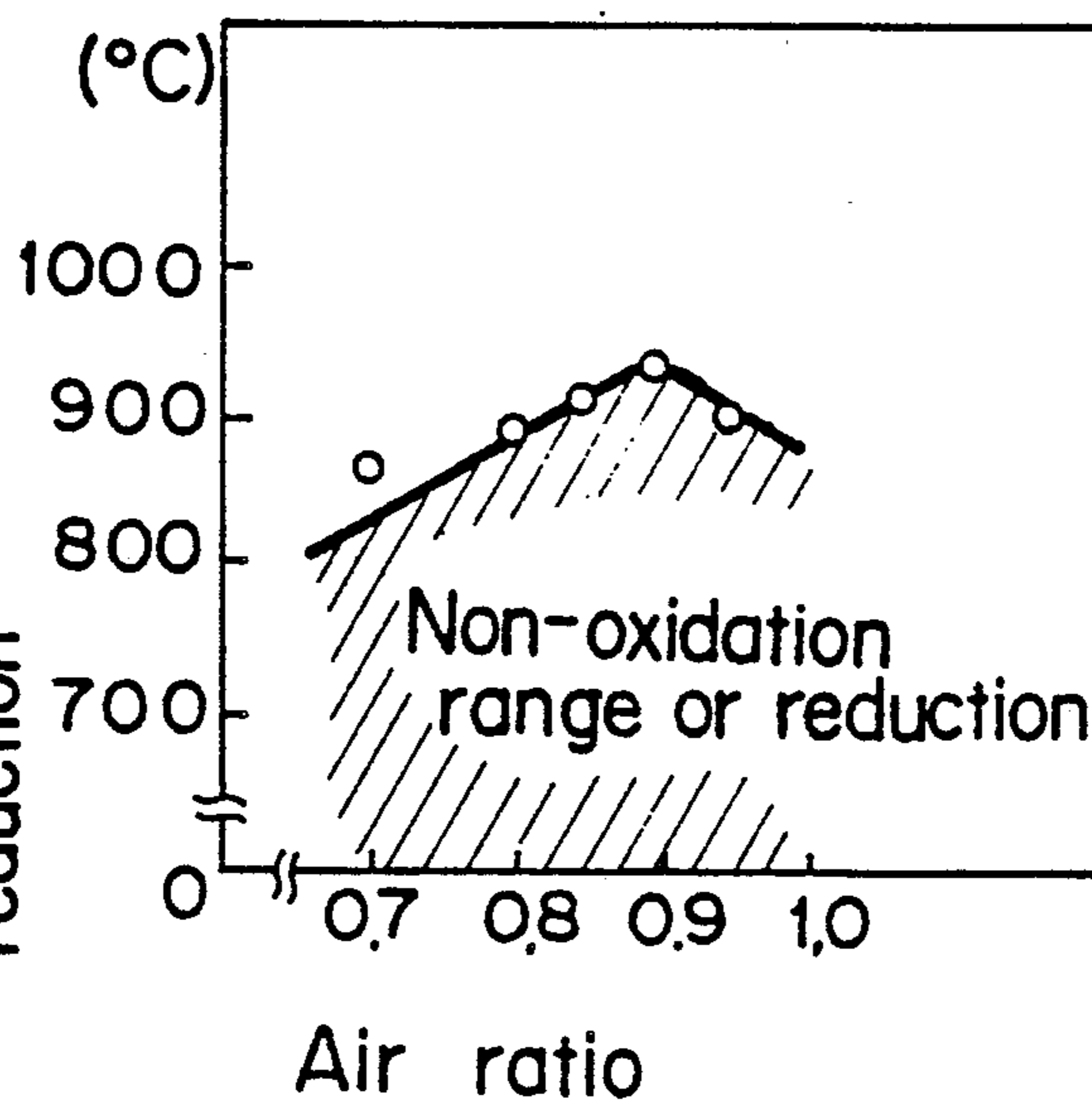
Limit temperature of heating without causing oxidation or with reduction
