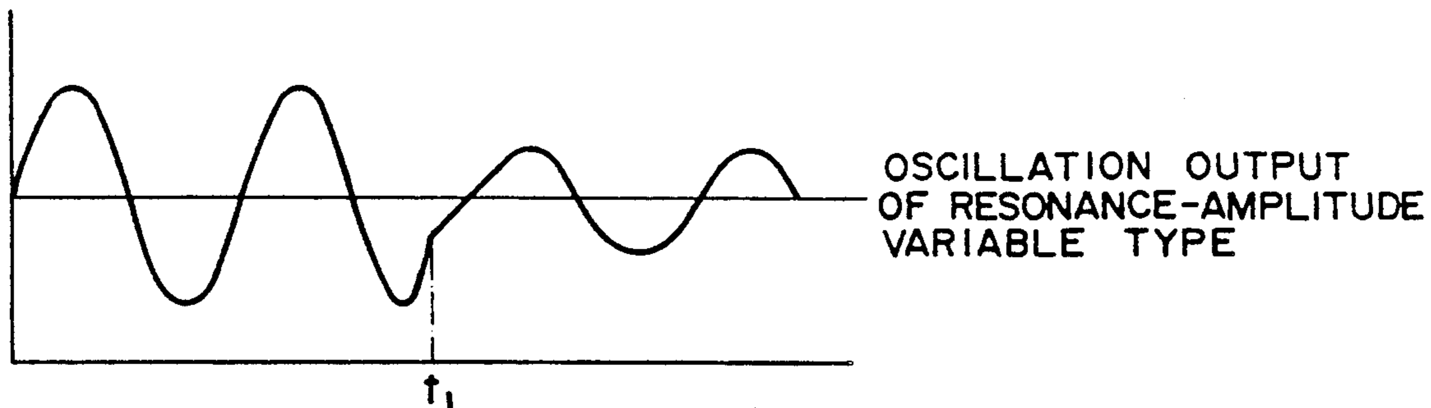
FIG. 18 PRIOR ART
