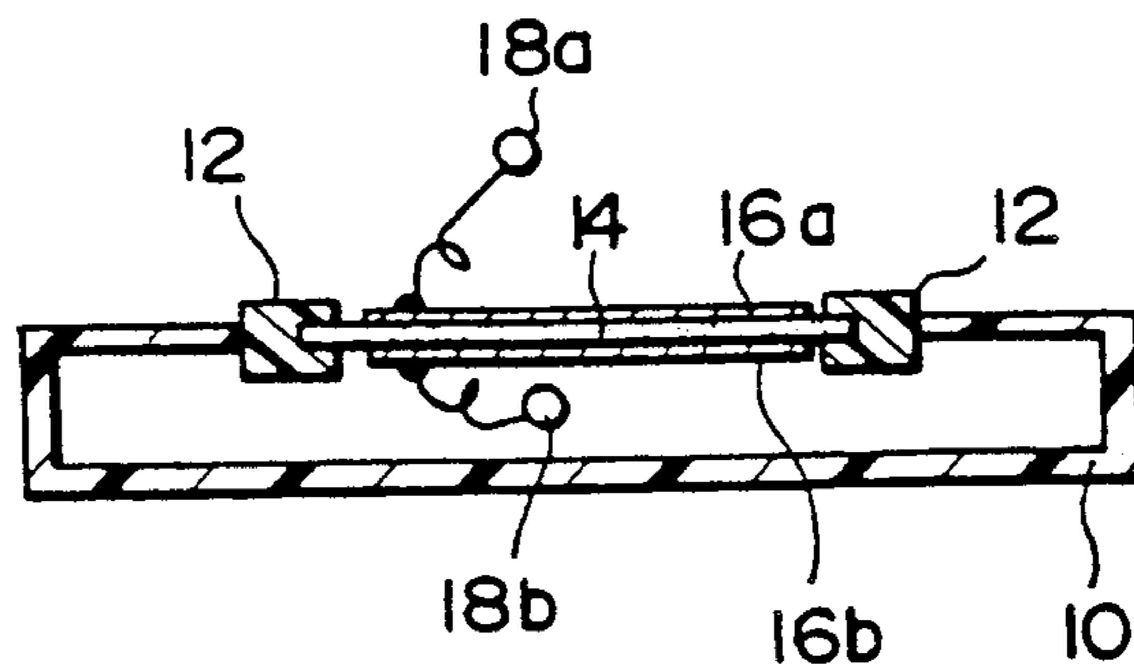
FIG. 13 PRIOR ART
