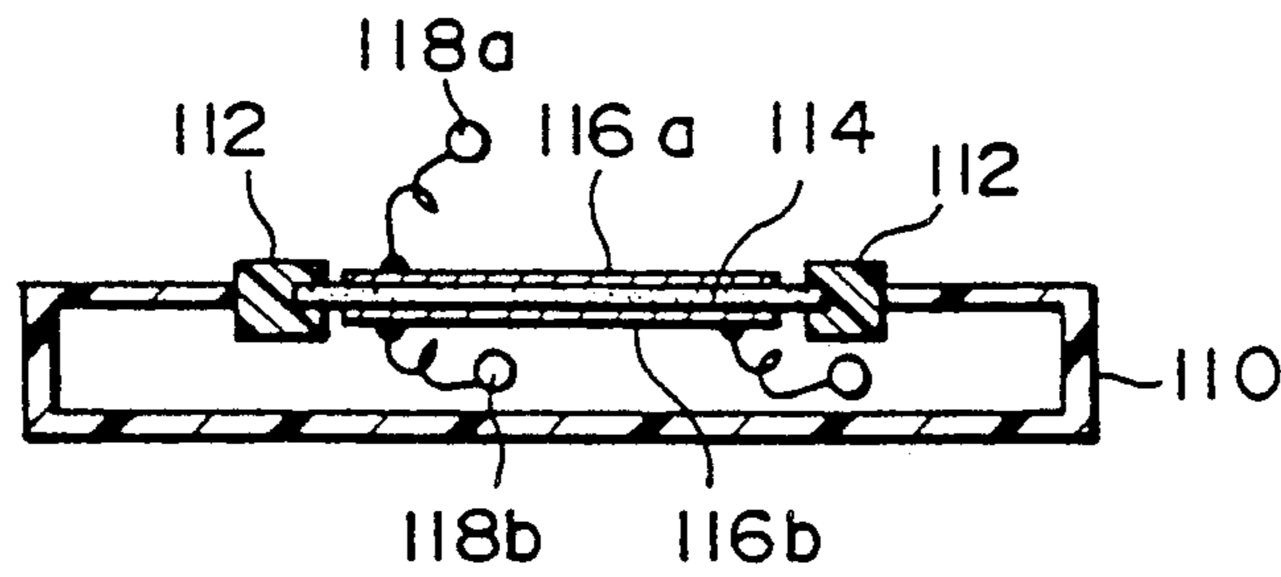
FIG. 15 PRIOR ART
