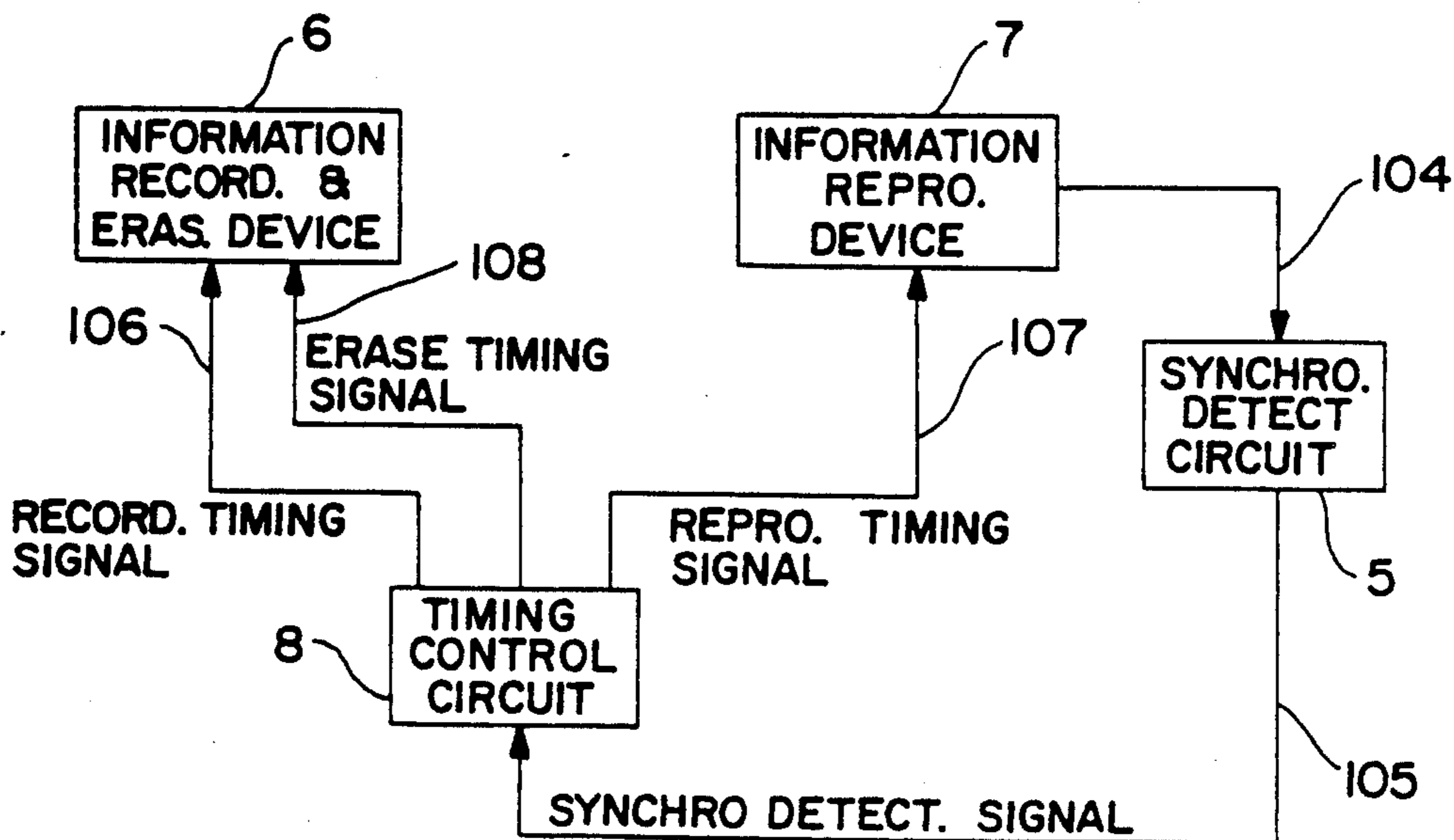
FIG. 3 PRIOR ART
