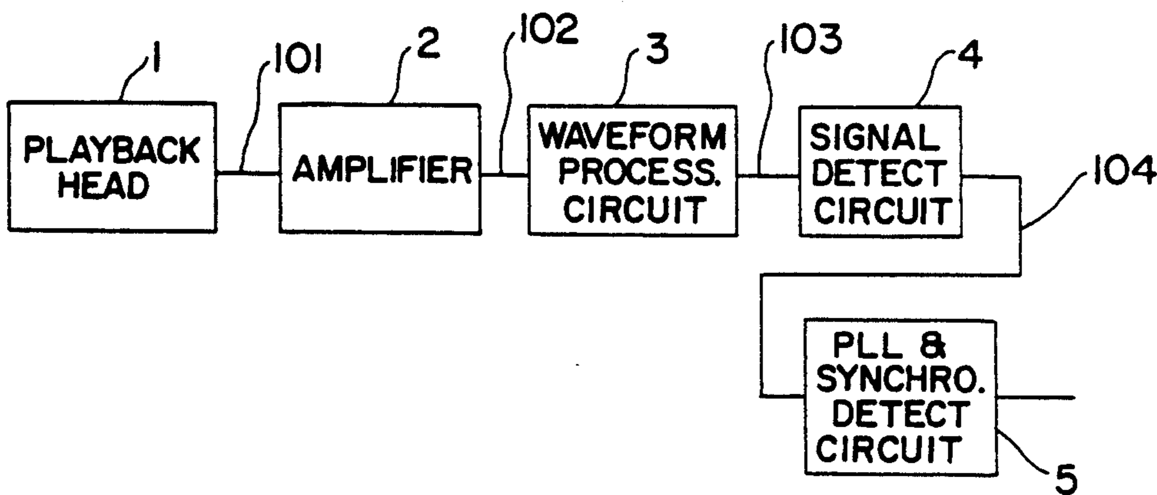
FIG. 2 PRIOR ART
