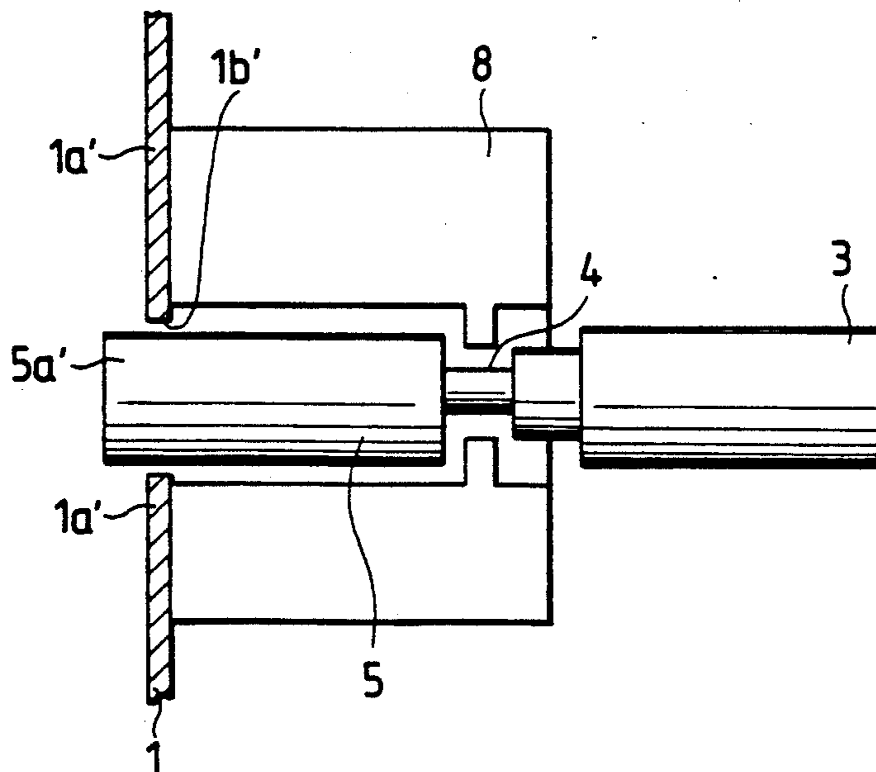
FIG. 13 PRIOR ART
