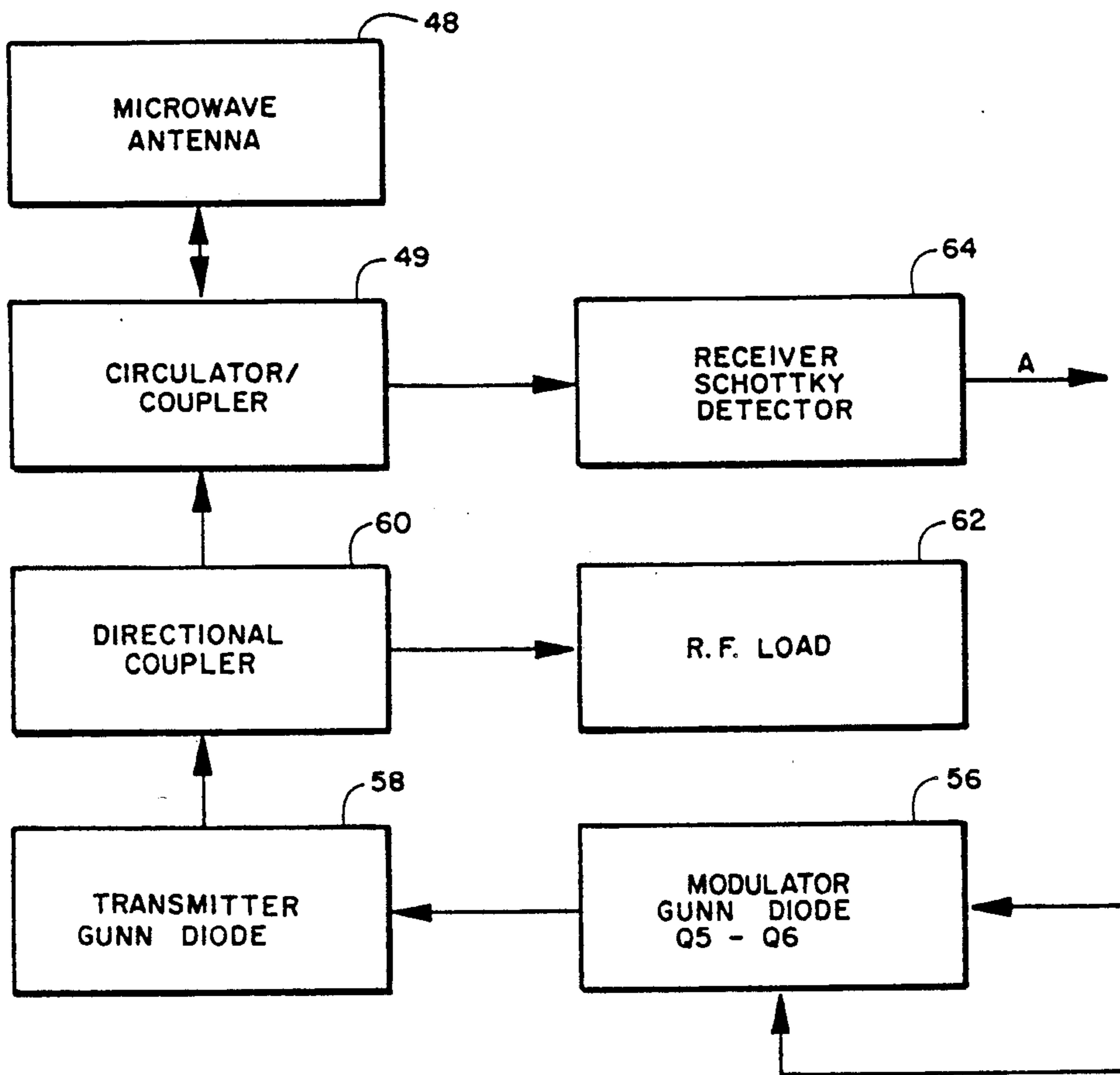
FIGURE 1 (PRIOR ART)
