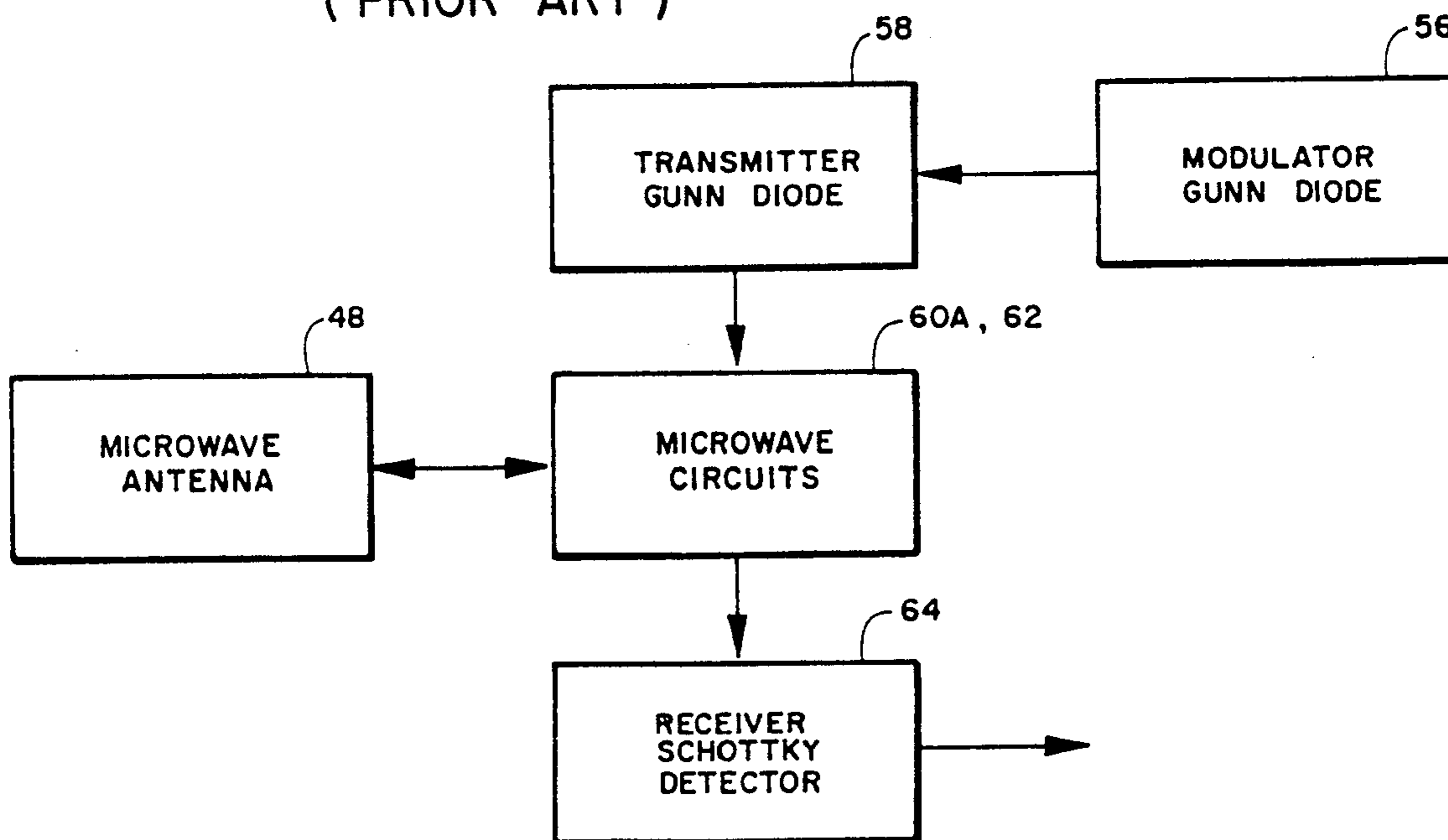
FIGURE 1 (PRIOR ART)
