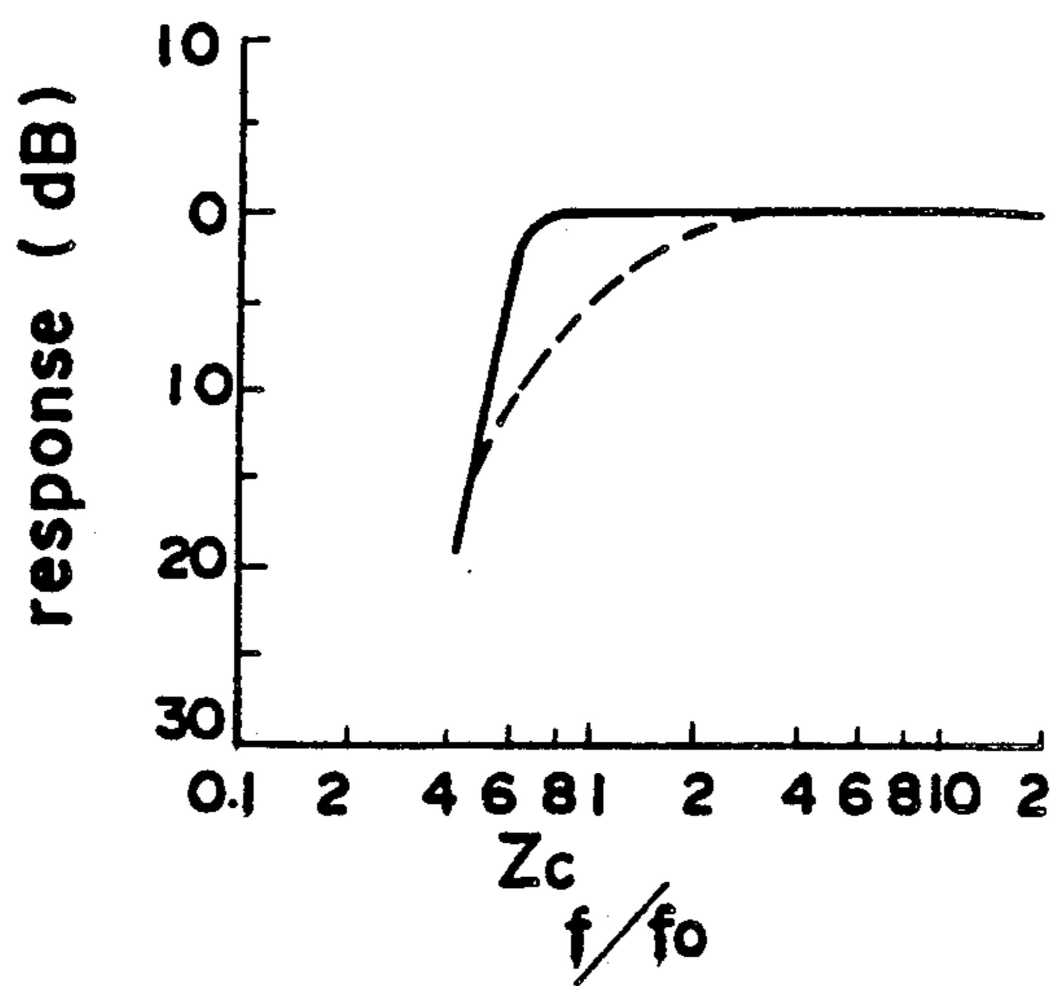
FIG. 12 (PRIOR ART)
