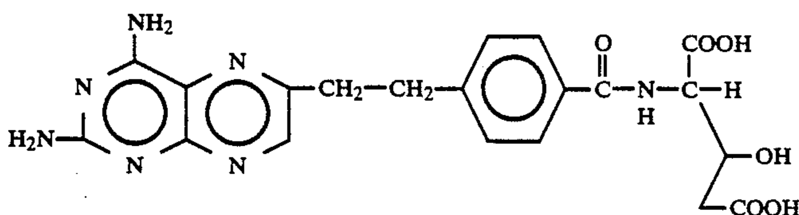
4-Amino-4-deoxy-10-deazapteroyl-3-hydroxyglutamic acid.
