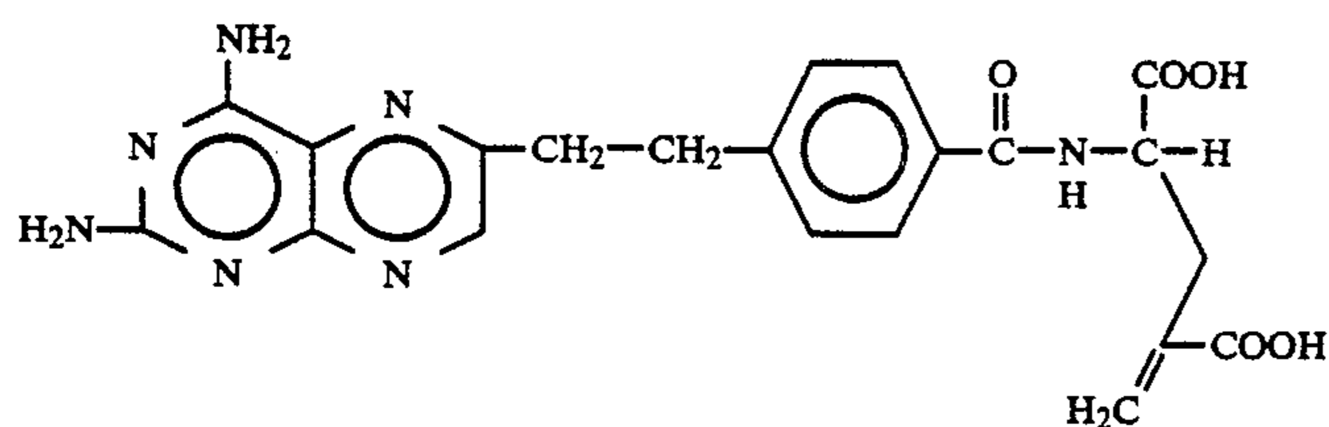
4-Amino-4-deoxy-10-deazapteroyl-gamma-methyleneglutamic acid.
