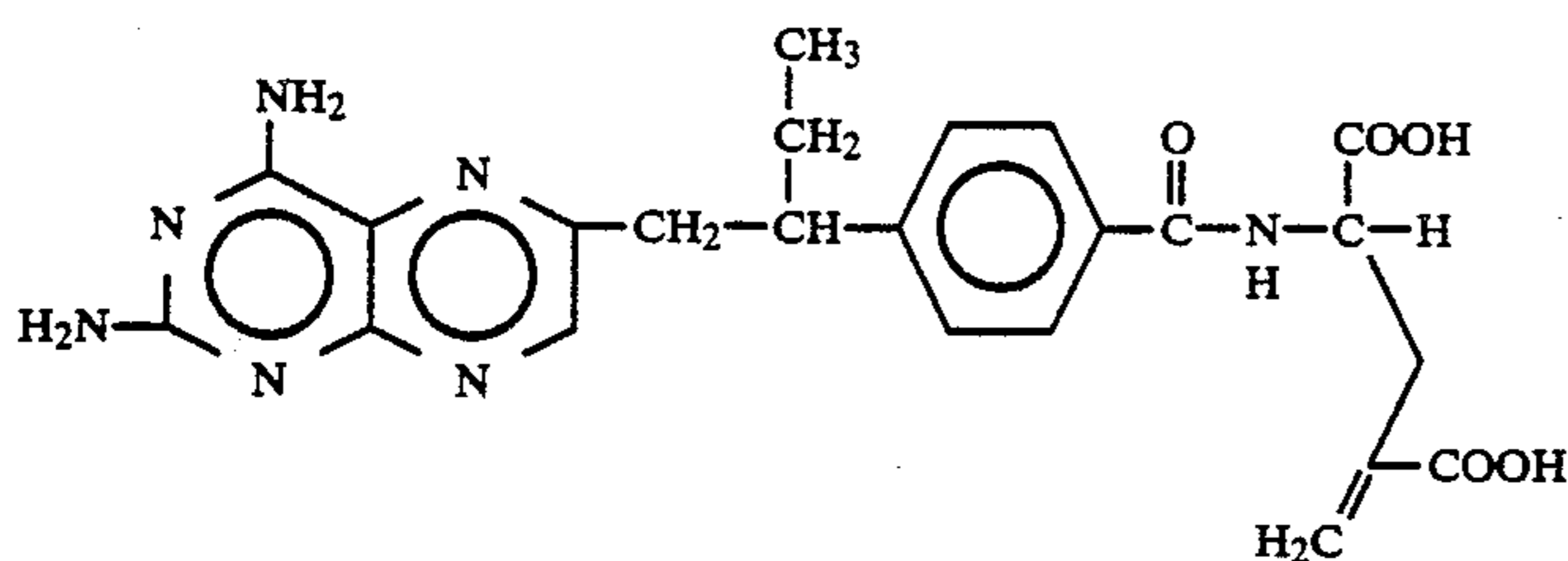
4-Amino-4-deoxy-10-ethyl-10-deazapteroyl-gamma-methyleneglutamic acid.
