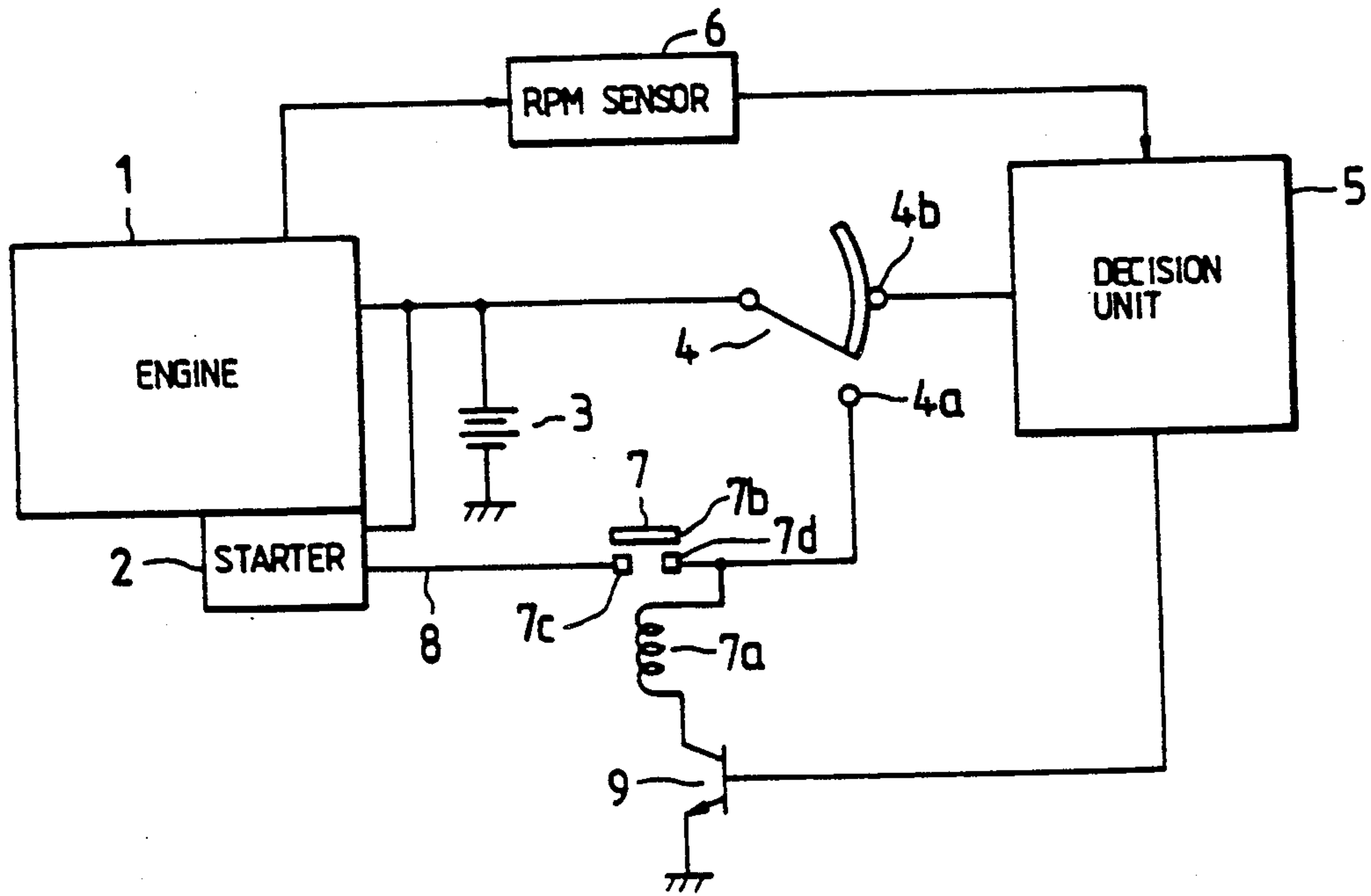
FIG. 3 PRIOR ART
