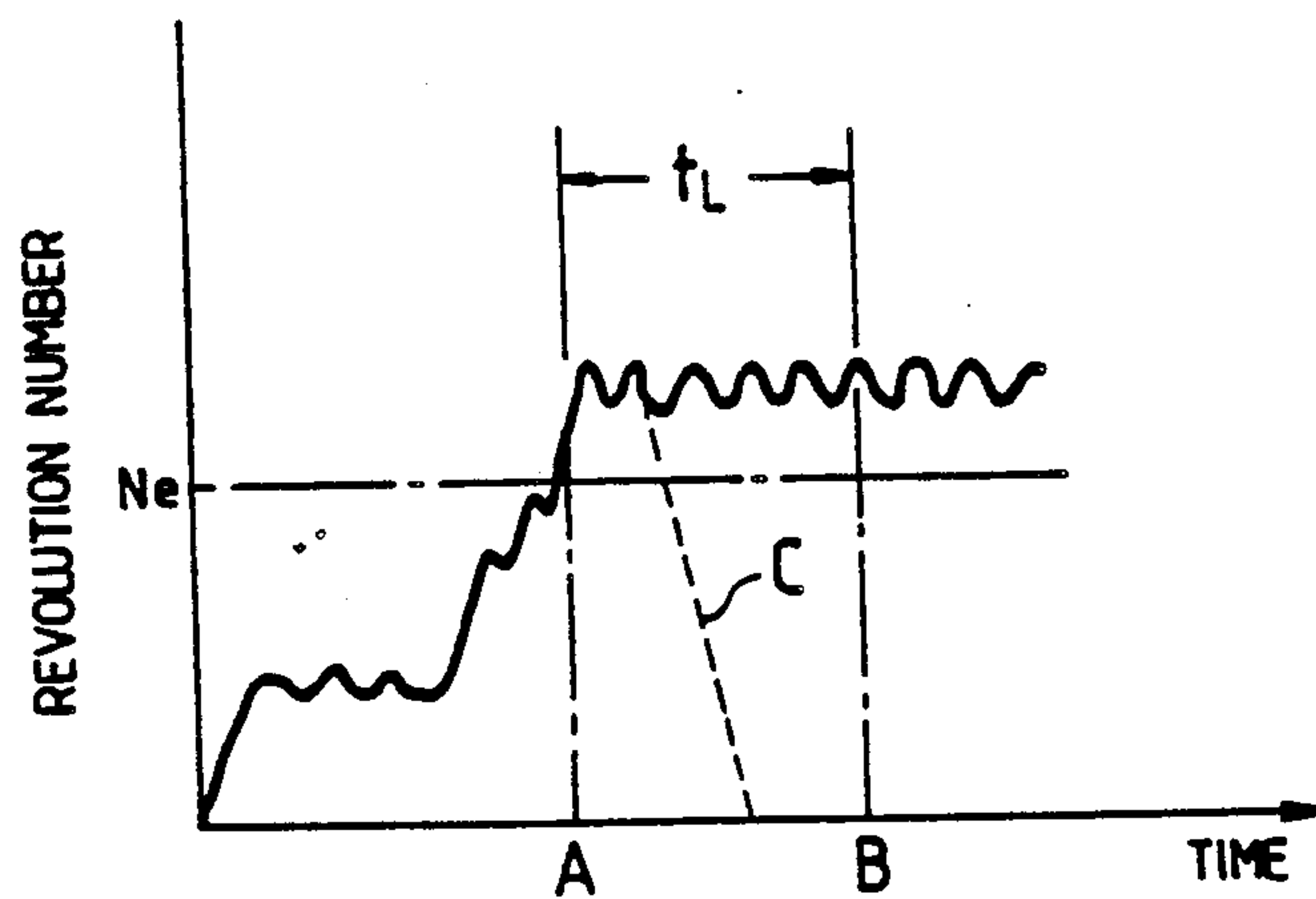
FIG. 4 PRIOR ART
