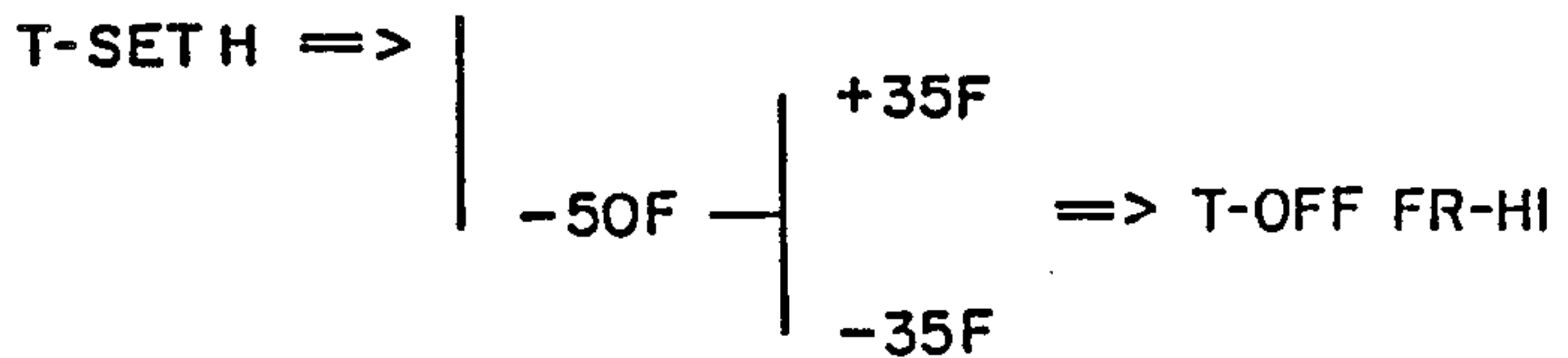
BAKE MODE FIRST RISE COMPENSATION ACTION POINTS.
