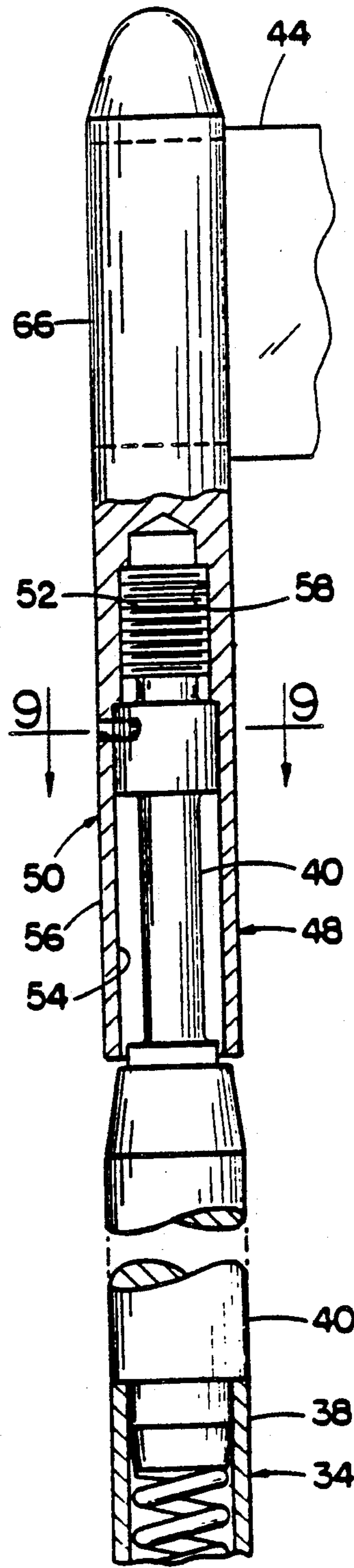
FIG. 8 (PRIOR ART)
