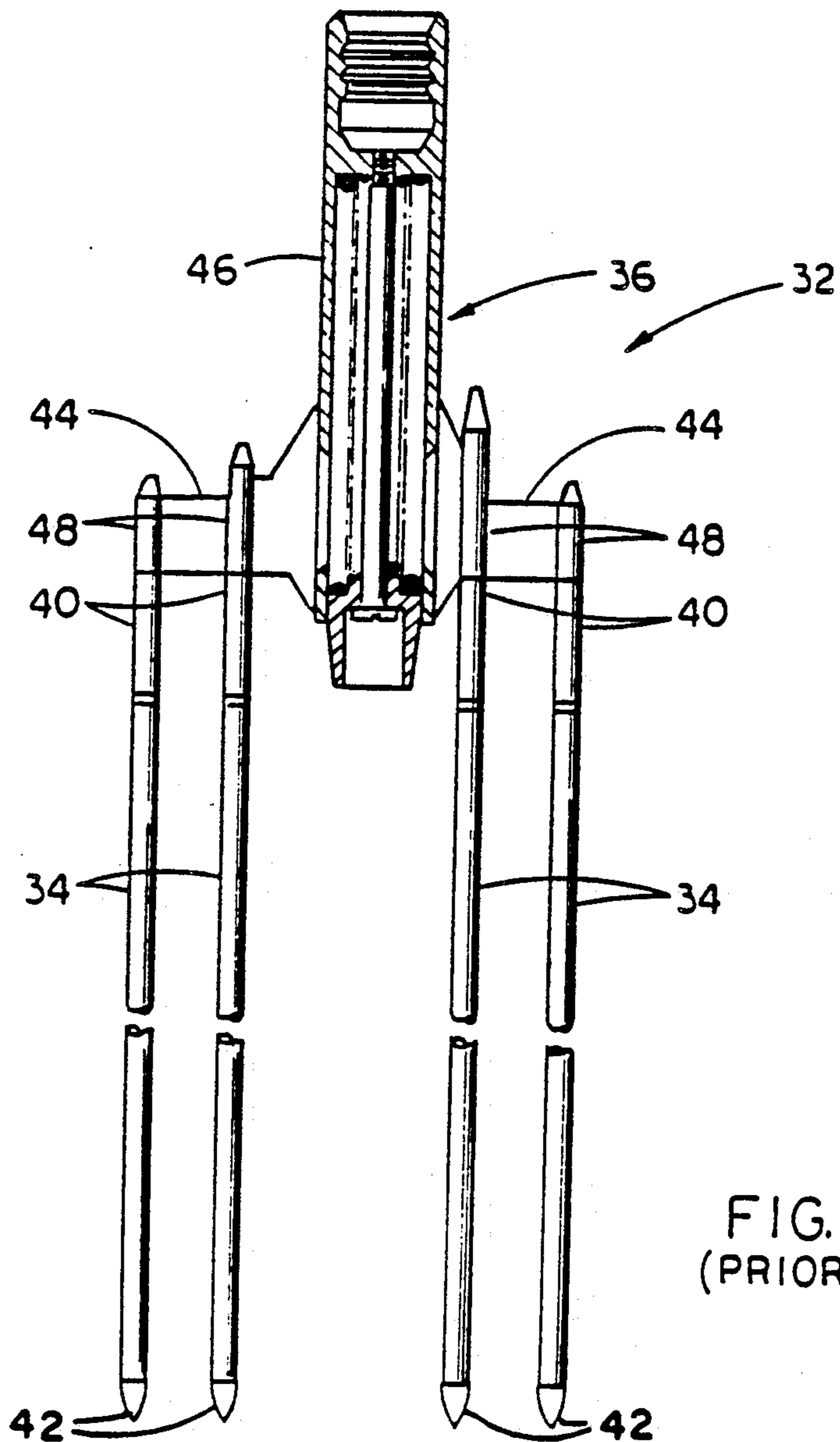
FIG. 2 (PRIOR ART)
