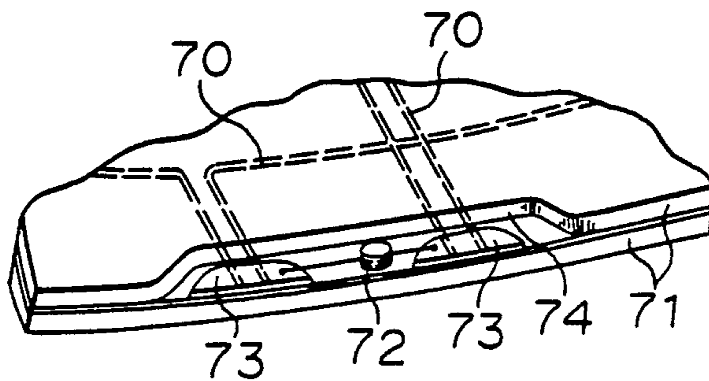
FIGURE 14 PRIOR ART
