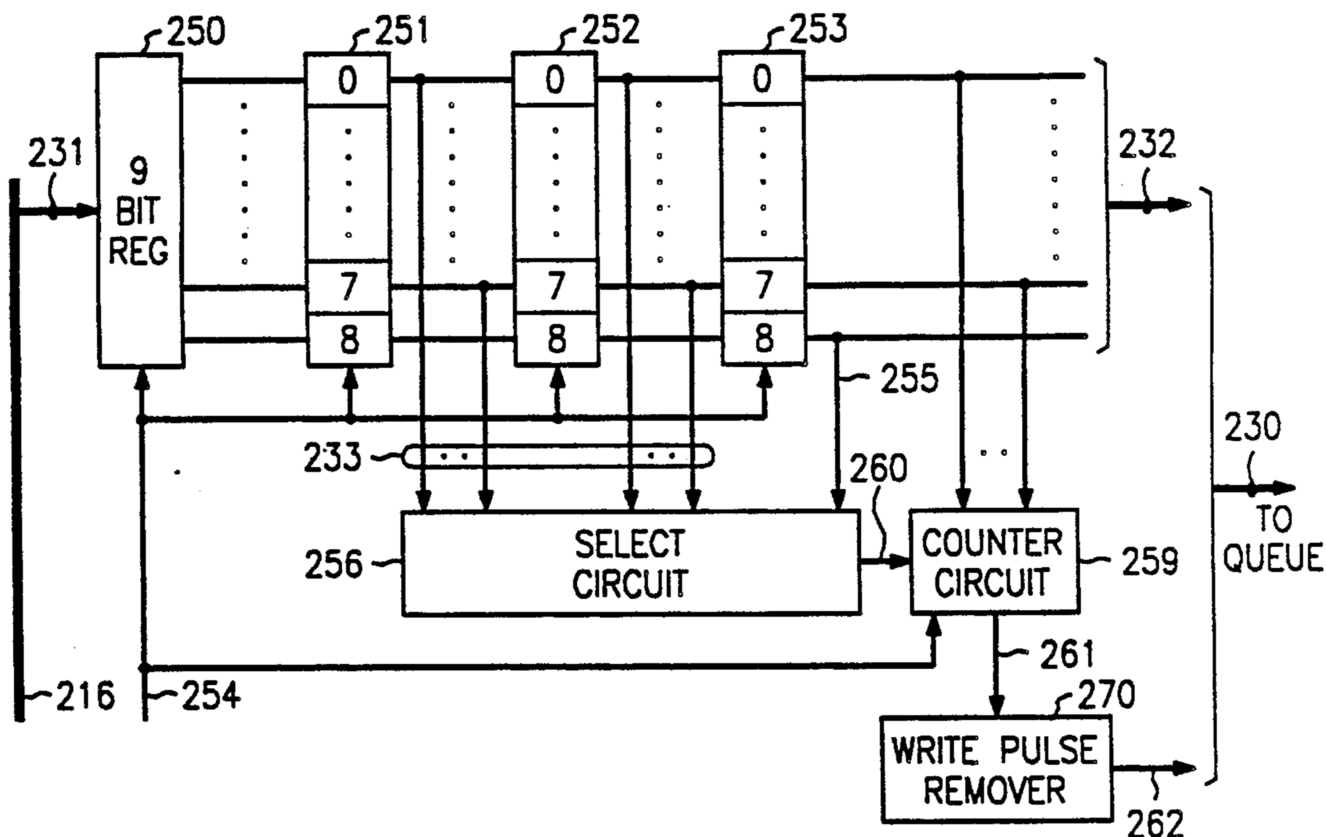
PACKET SELECT
