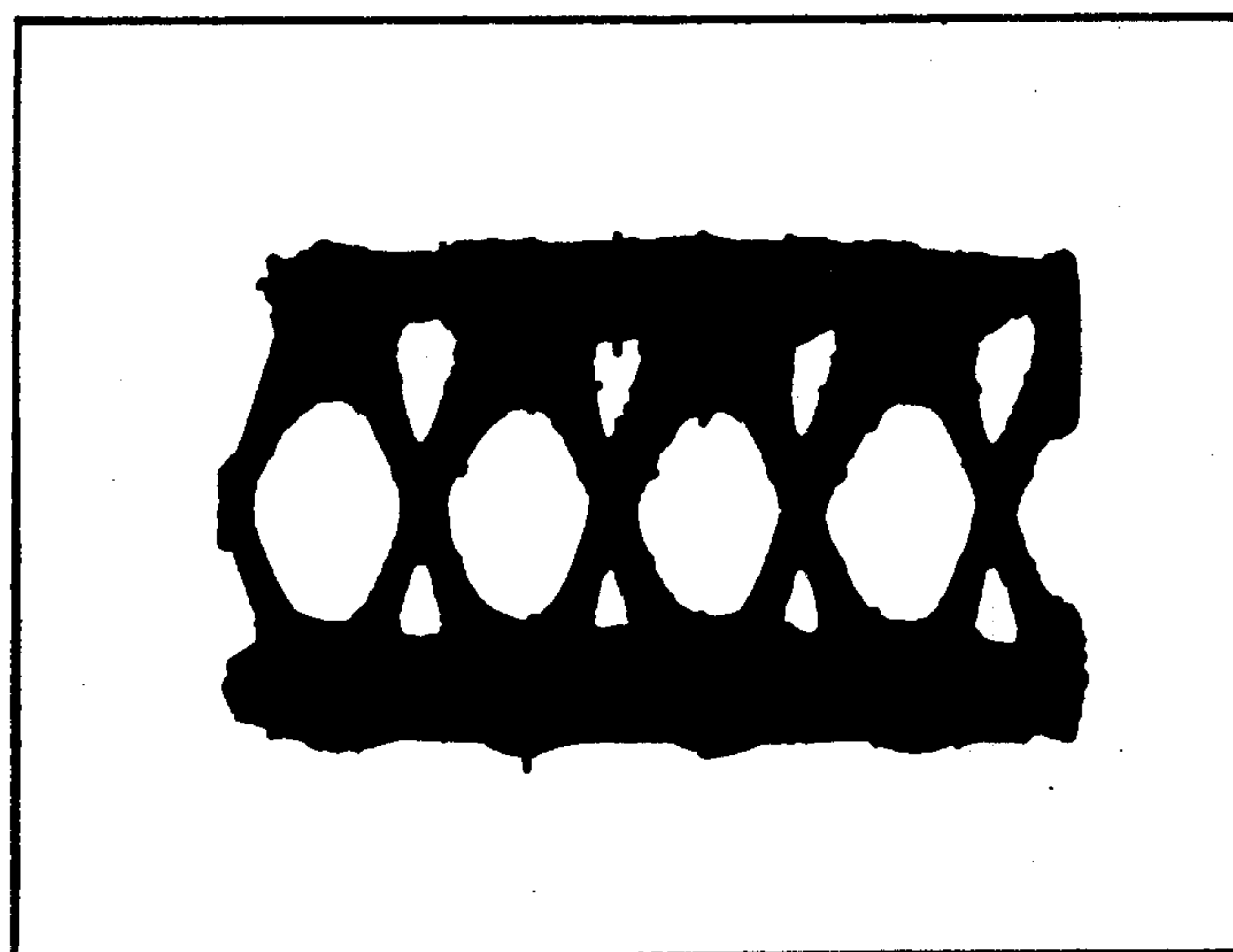
TWO CHANNELS SPACED AT 100 MHz
