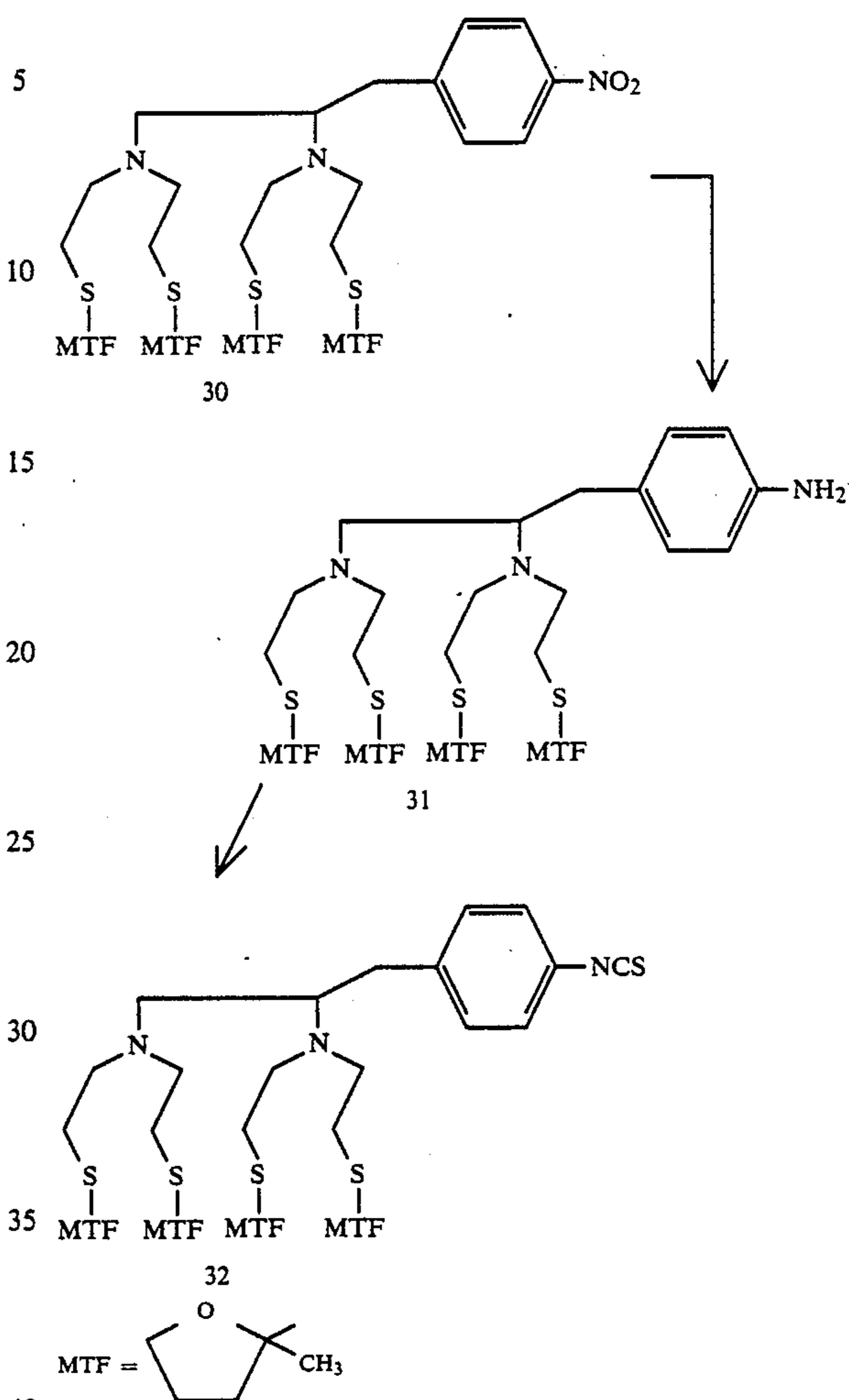
-continued SCHEME 4
