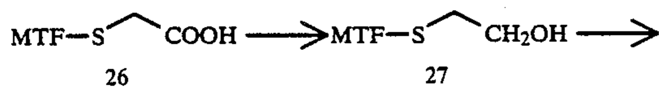
SCHEME 4
