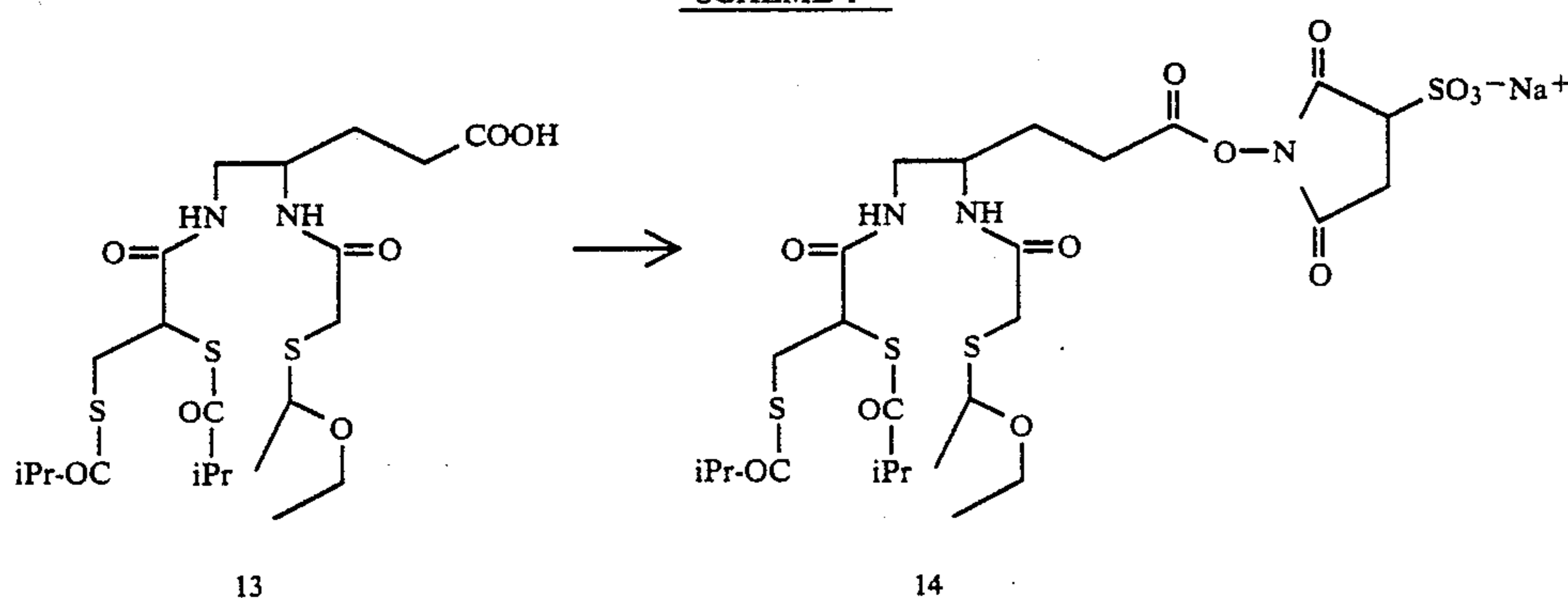
SCHEME 1
