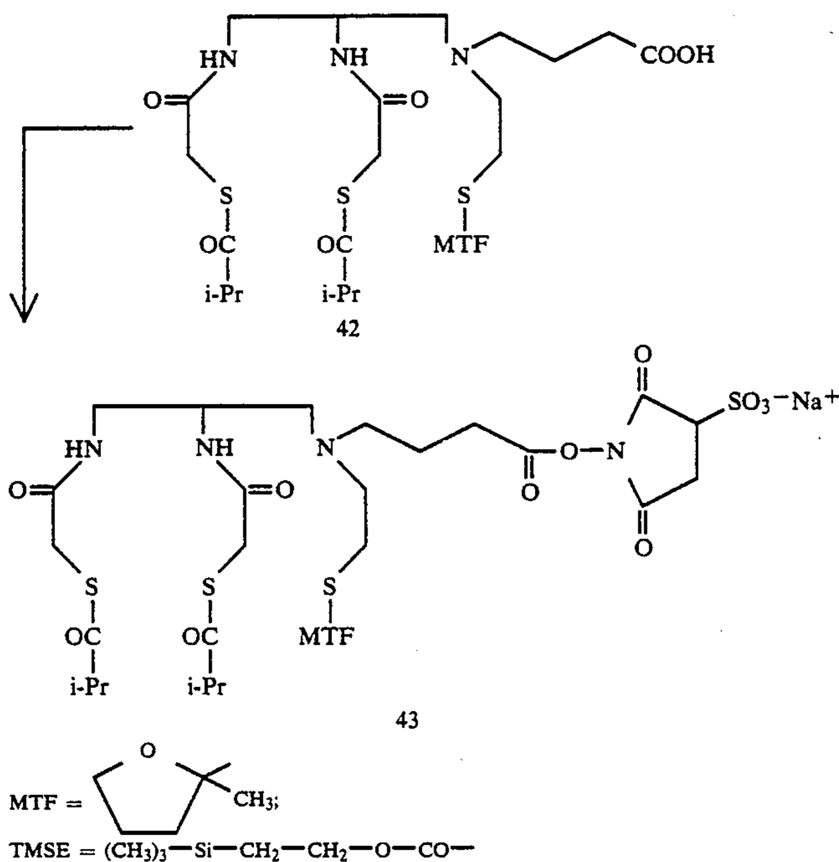
SCHEME 5
