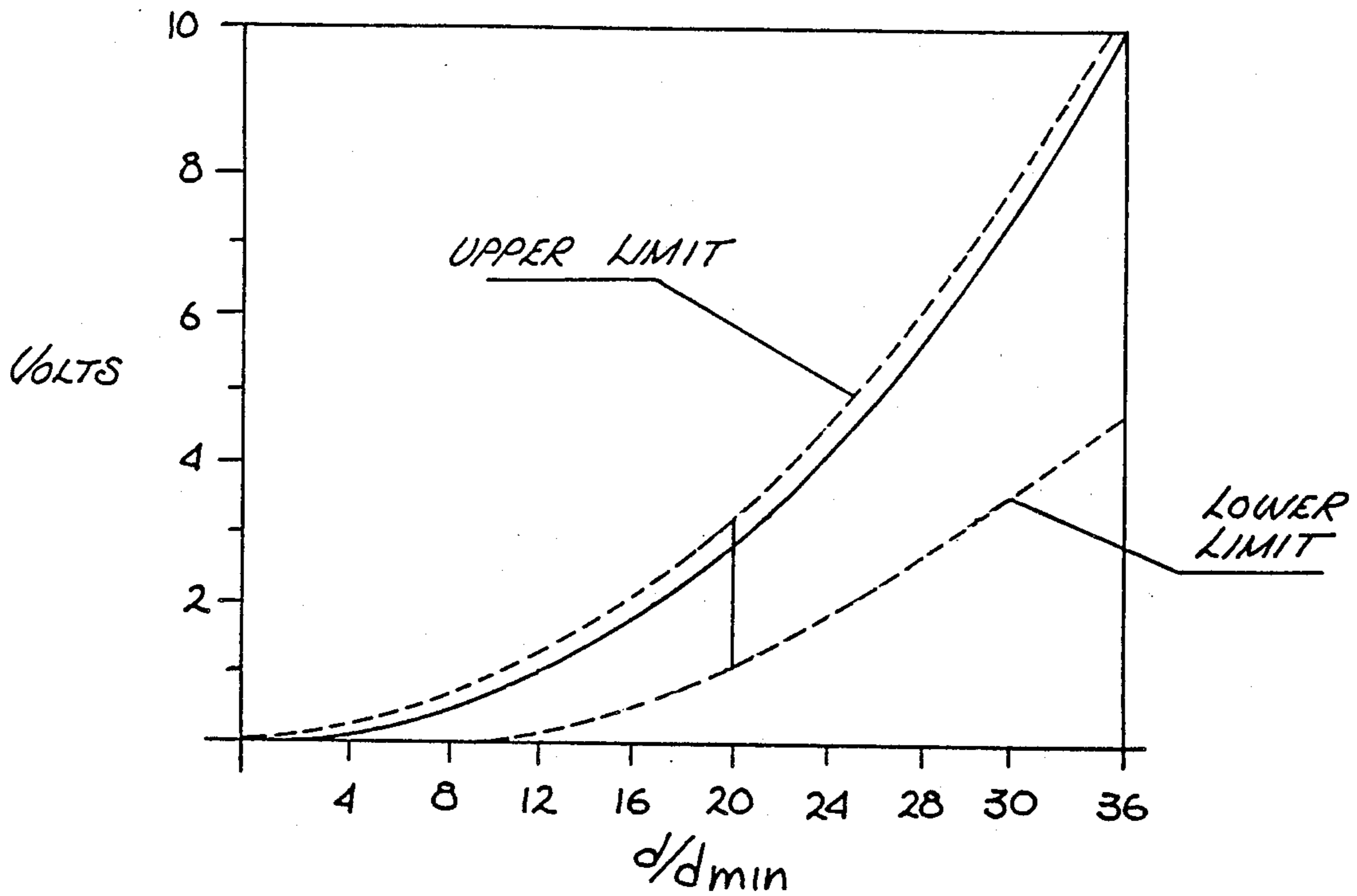
SIGNAL VOLTAGE VARIATION WITH PARTICLE SIZE Fig. 5
