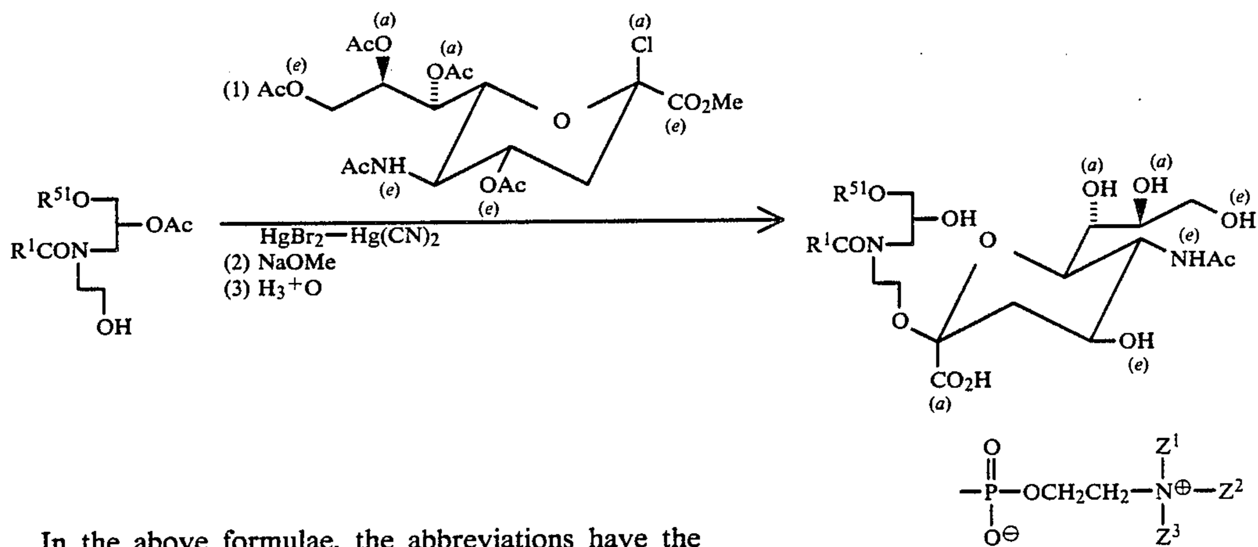
(7) Reaction making use of N-acetylneuraminic acid:
