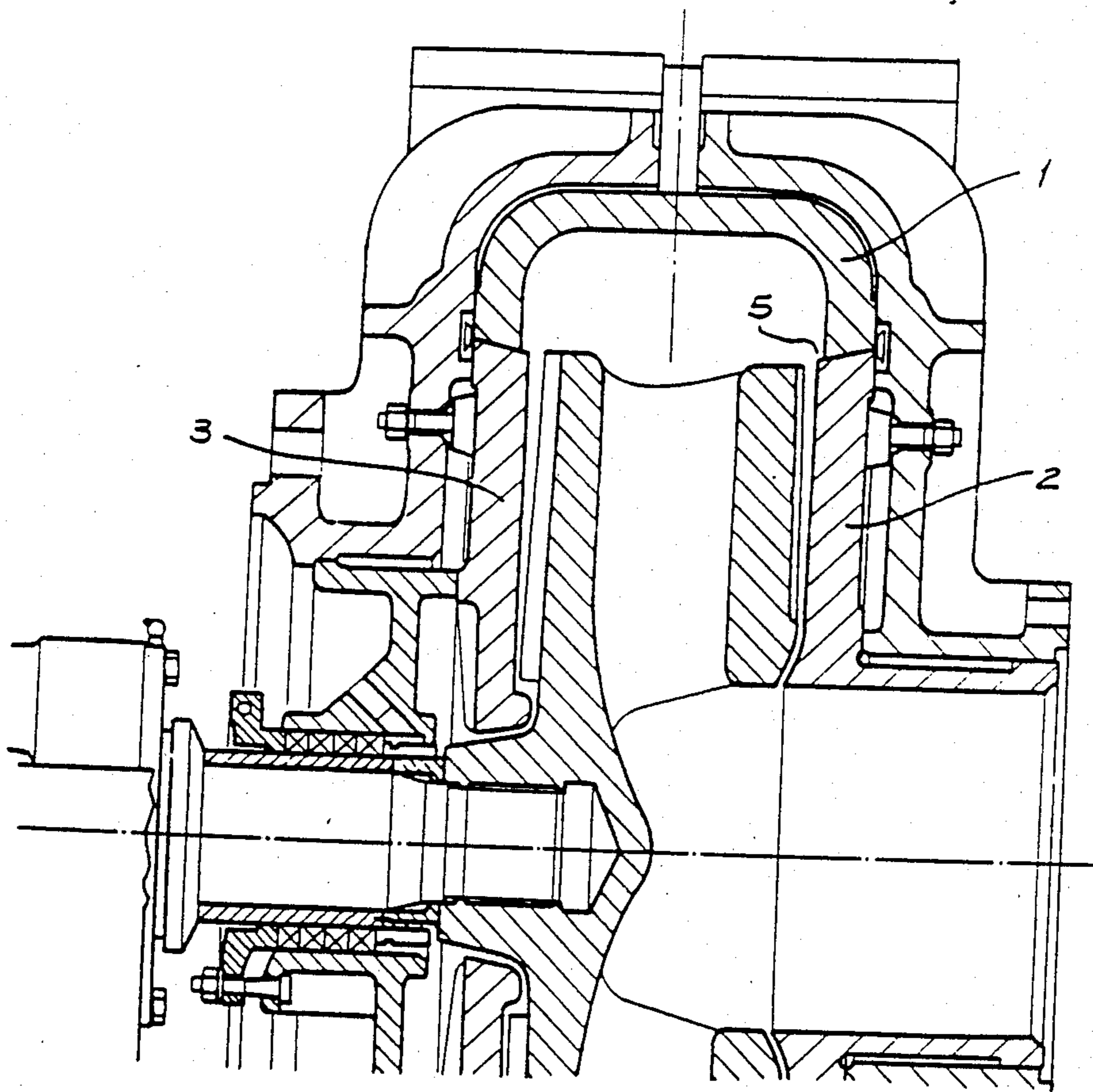
FIG. 3 PRIOR ART
