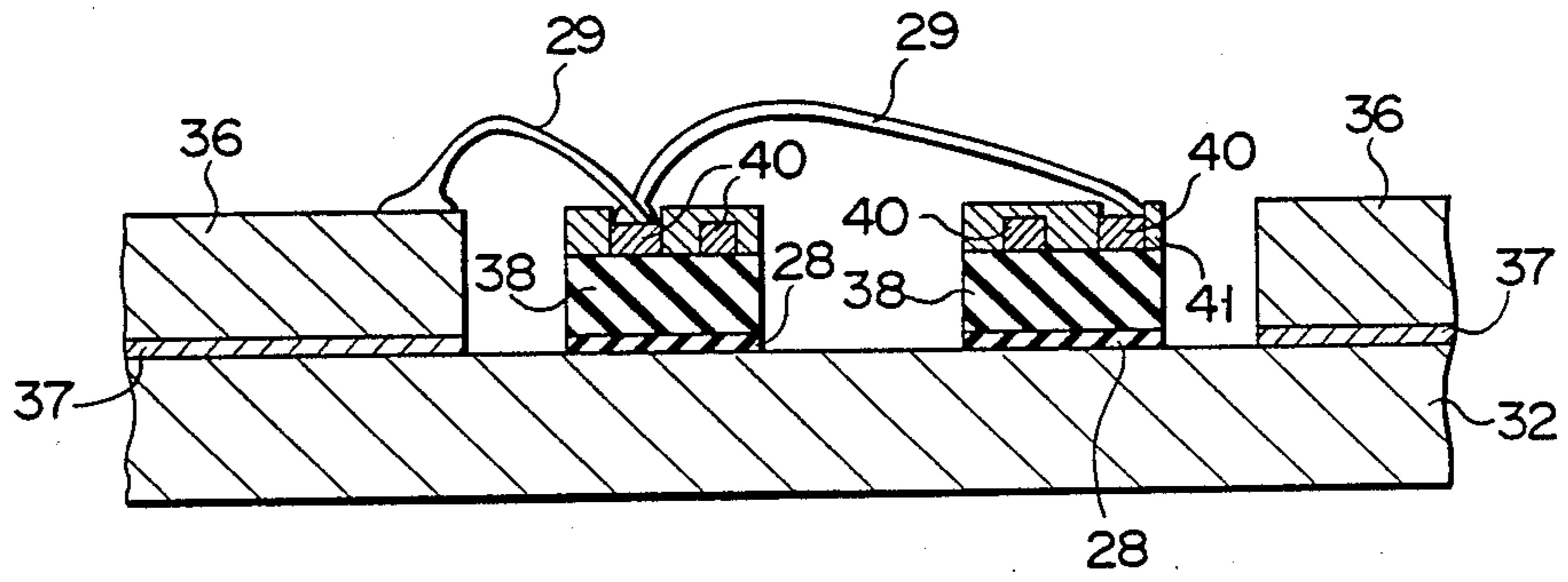
FIG. 2 PRIOR ART
