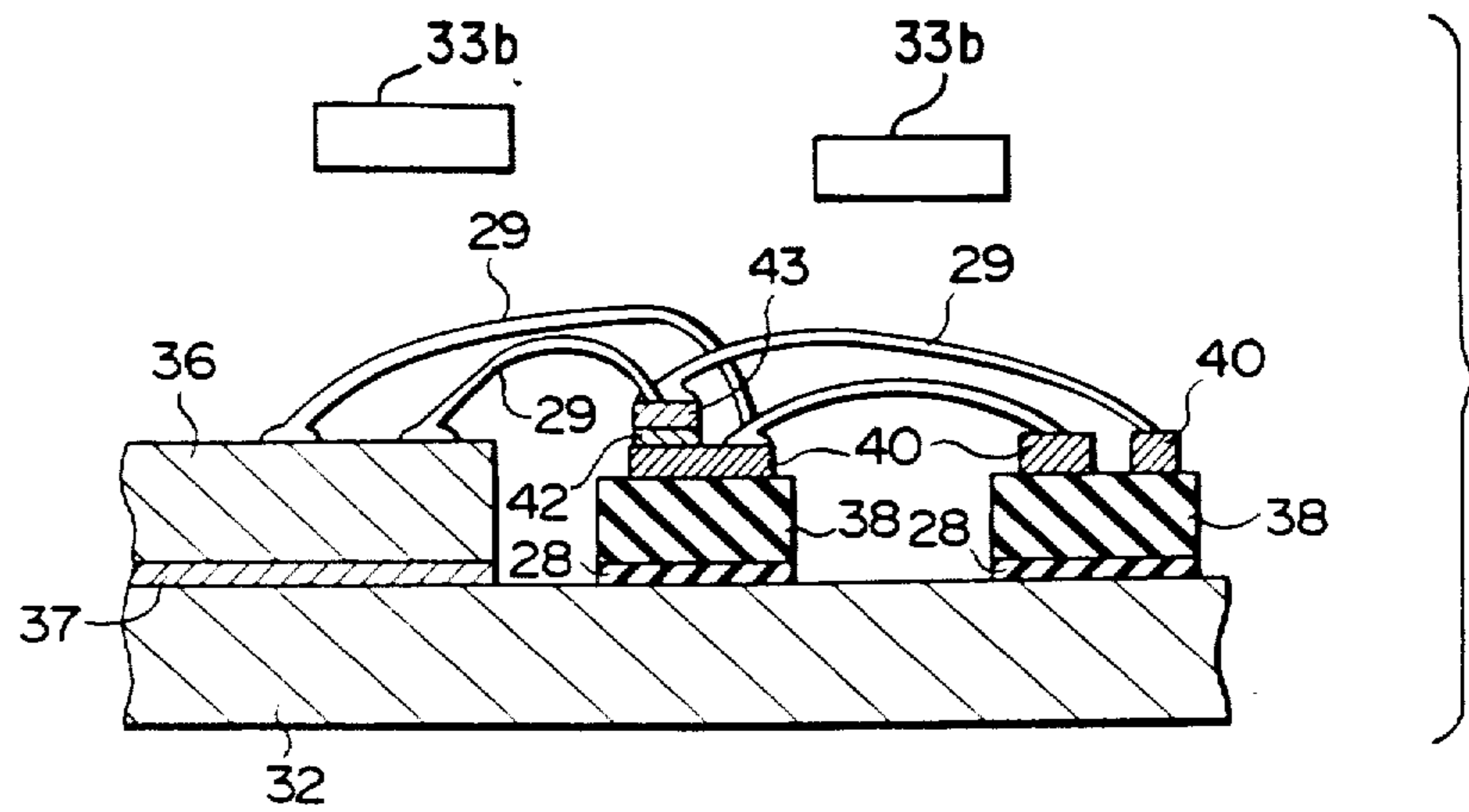
FIG. 3 PRIOR ART
