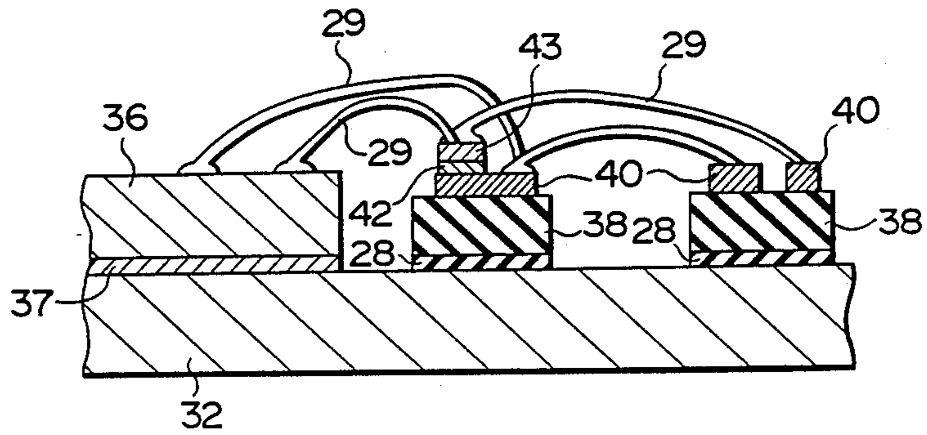
FIG. 3 PRIOR ART
