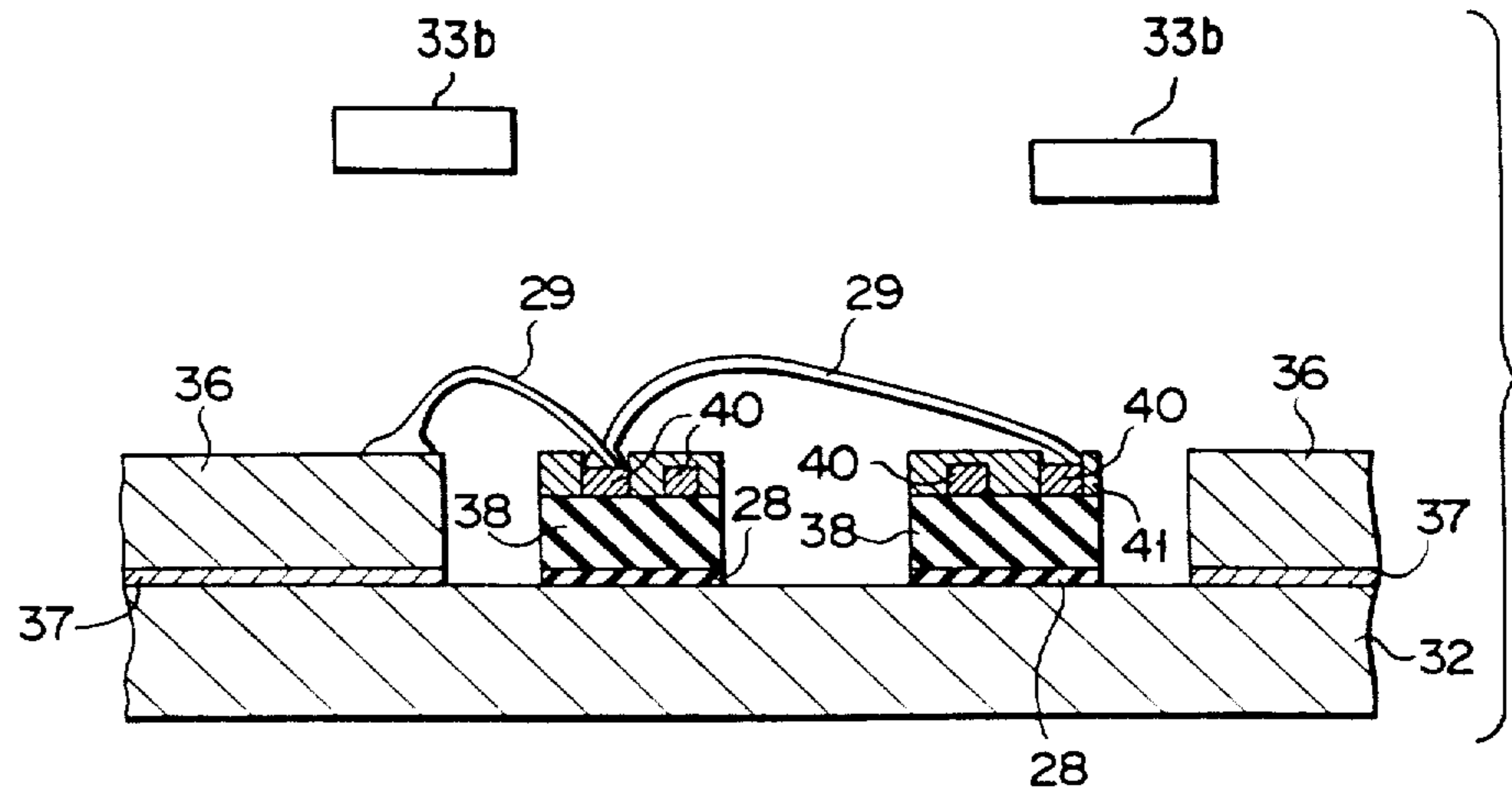
FIG. 2 PRIOR ART
