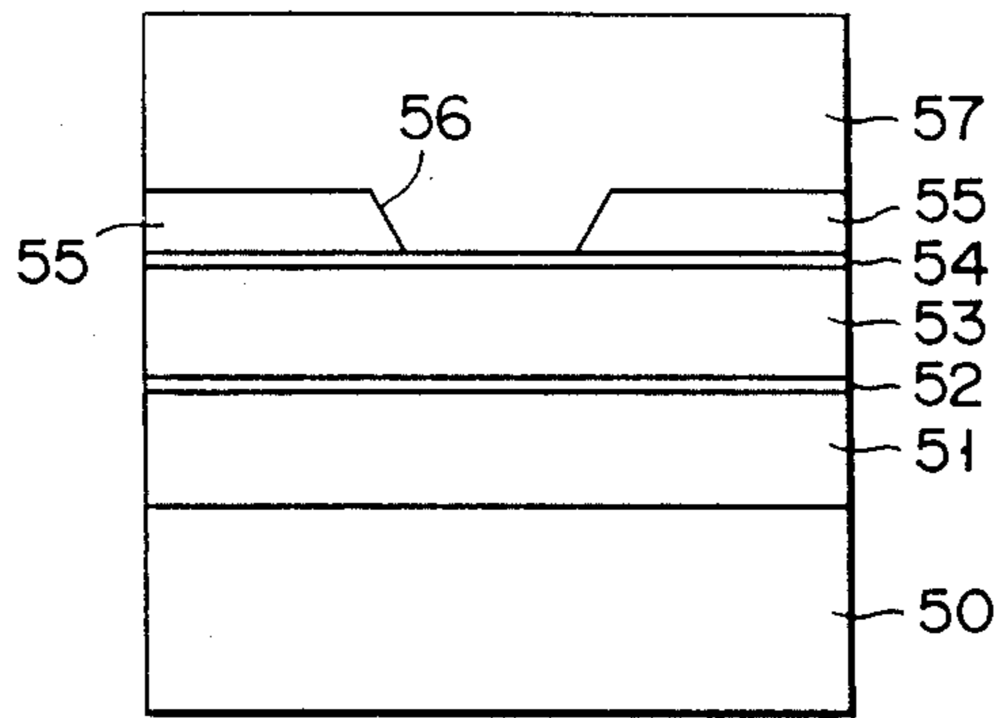
FIG. 1 (PRIOR ART)
