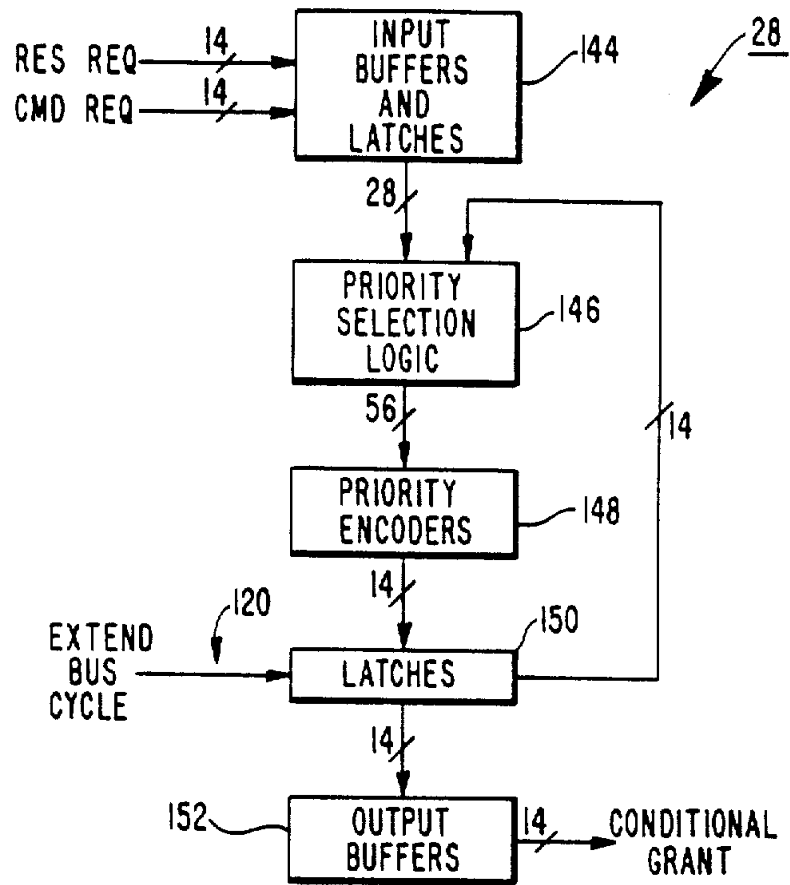
ARBITER BLOCK DIAGRAM
