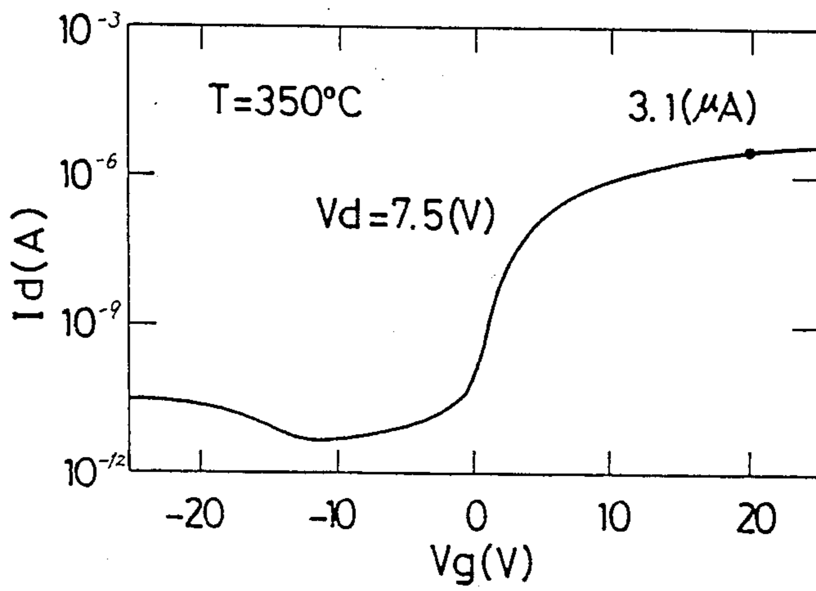
FIG. 6 PRIOR ART
