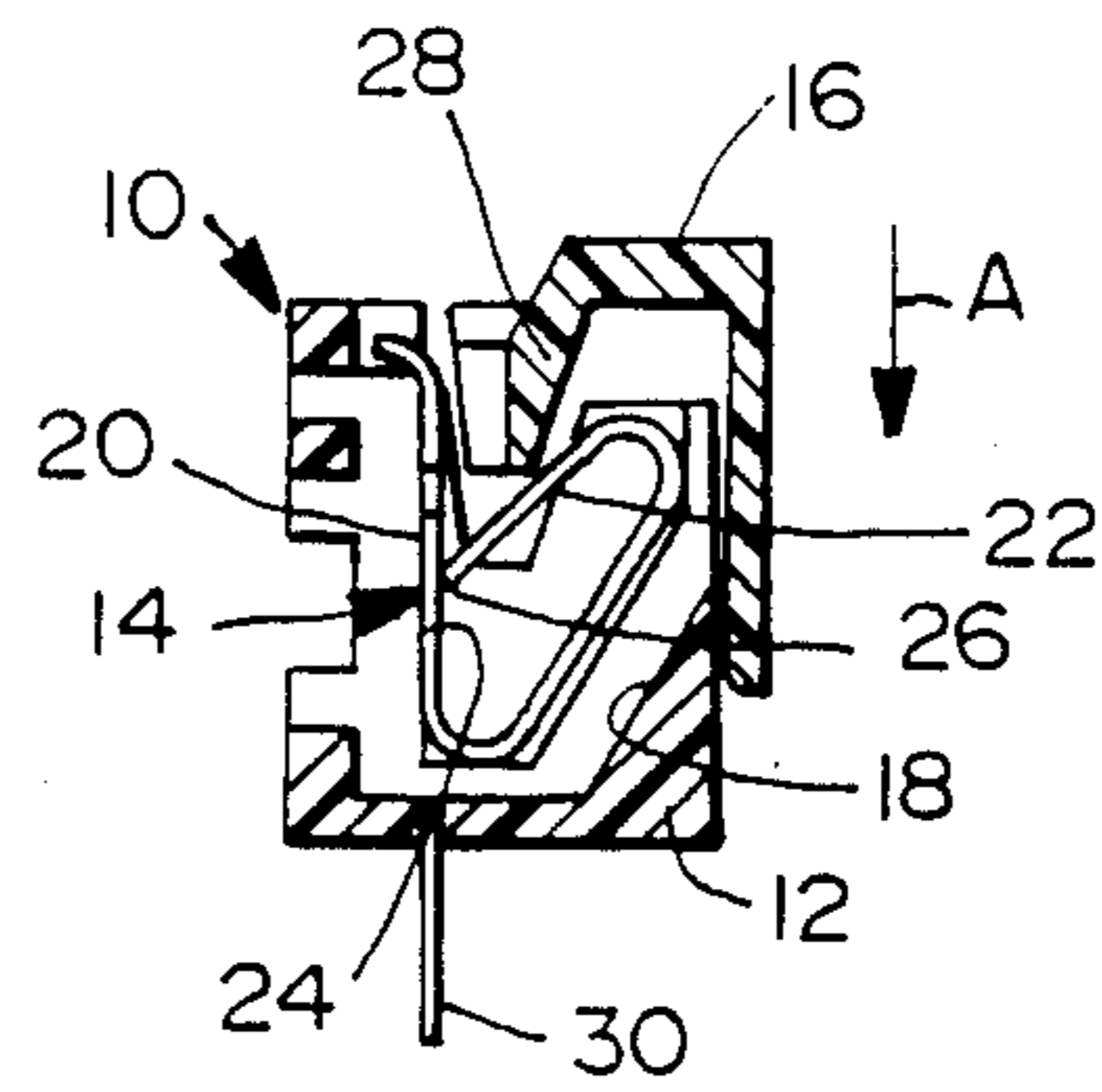
FIG. 1 (PRIOR ART)
