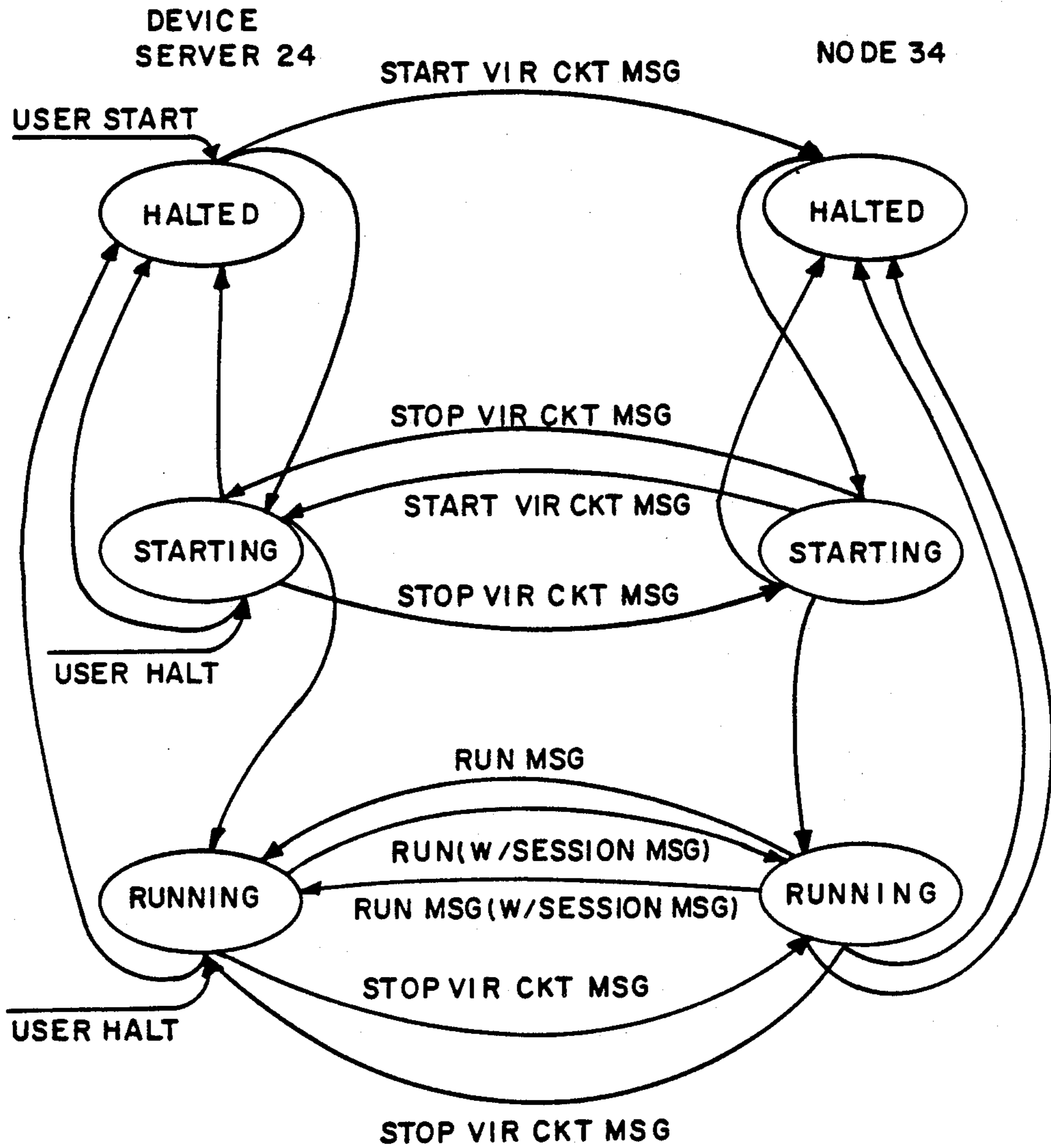
VIRTUAL CIRCUIT STATE DIAGRAM
