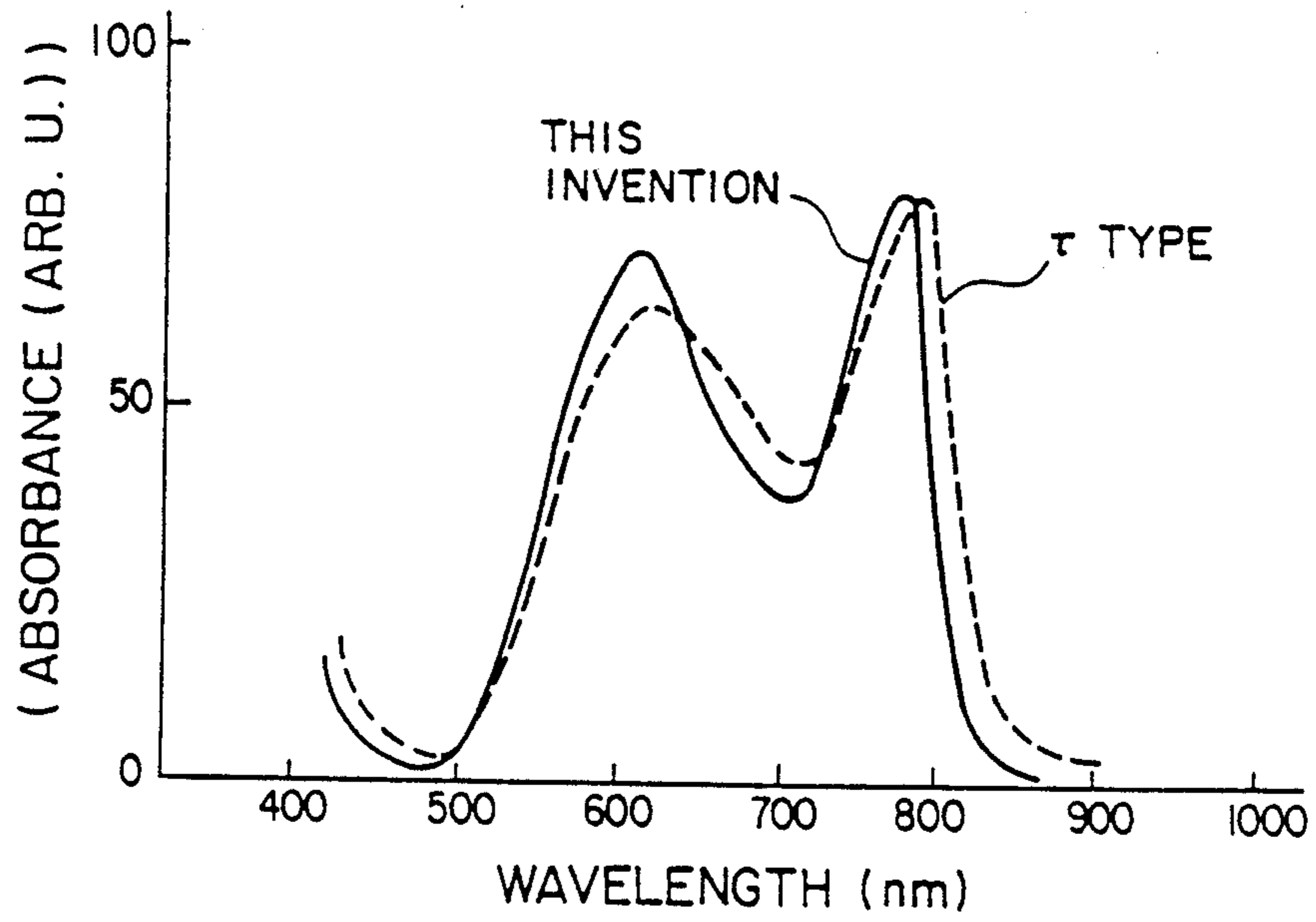
NEAR-INFRARED ABSORPTION SPECTRUM
