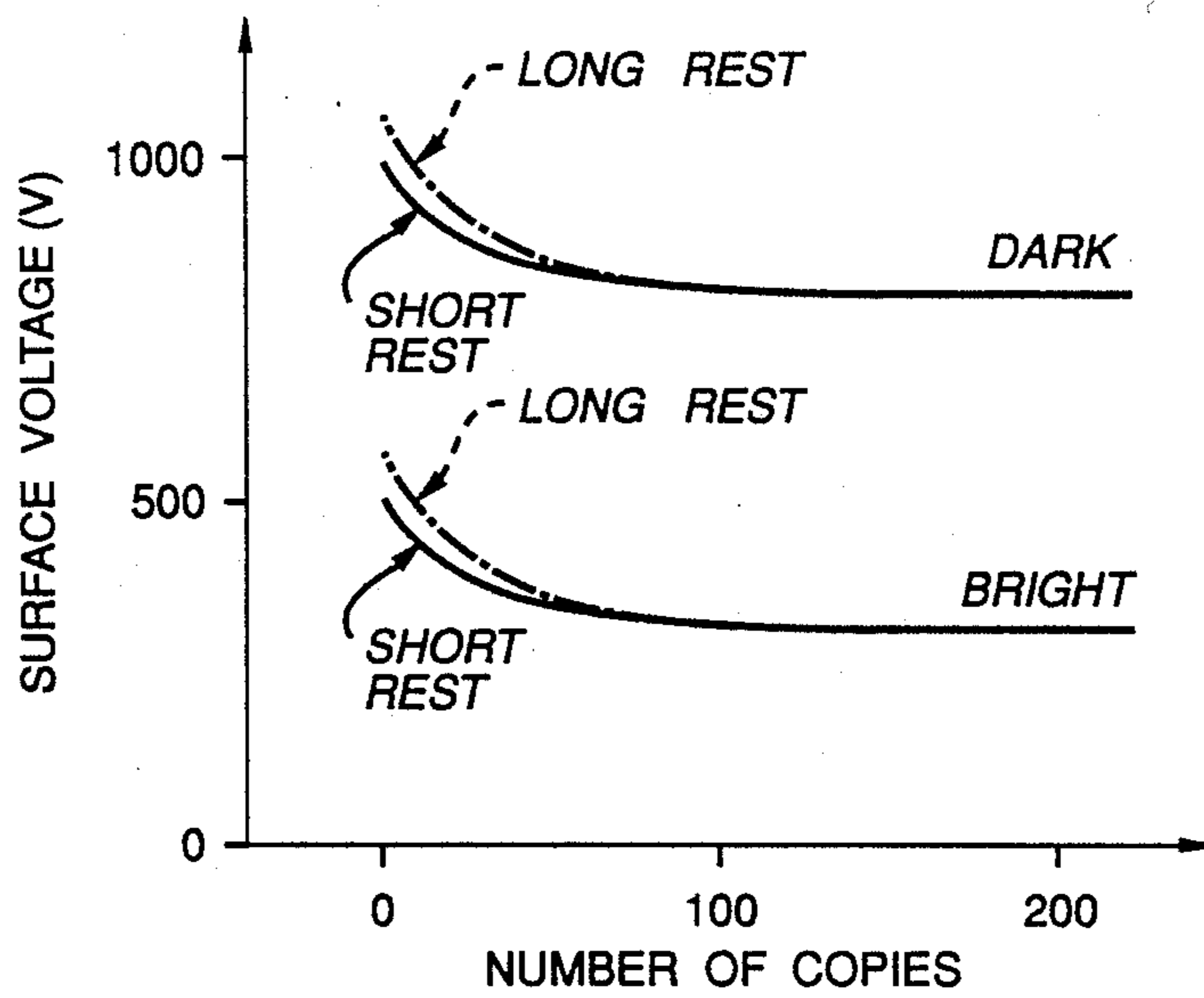
FIG. 1 (PRIOR ART)
