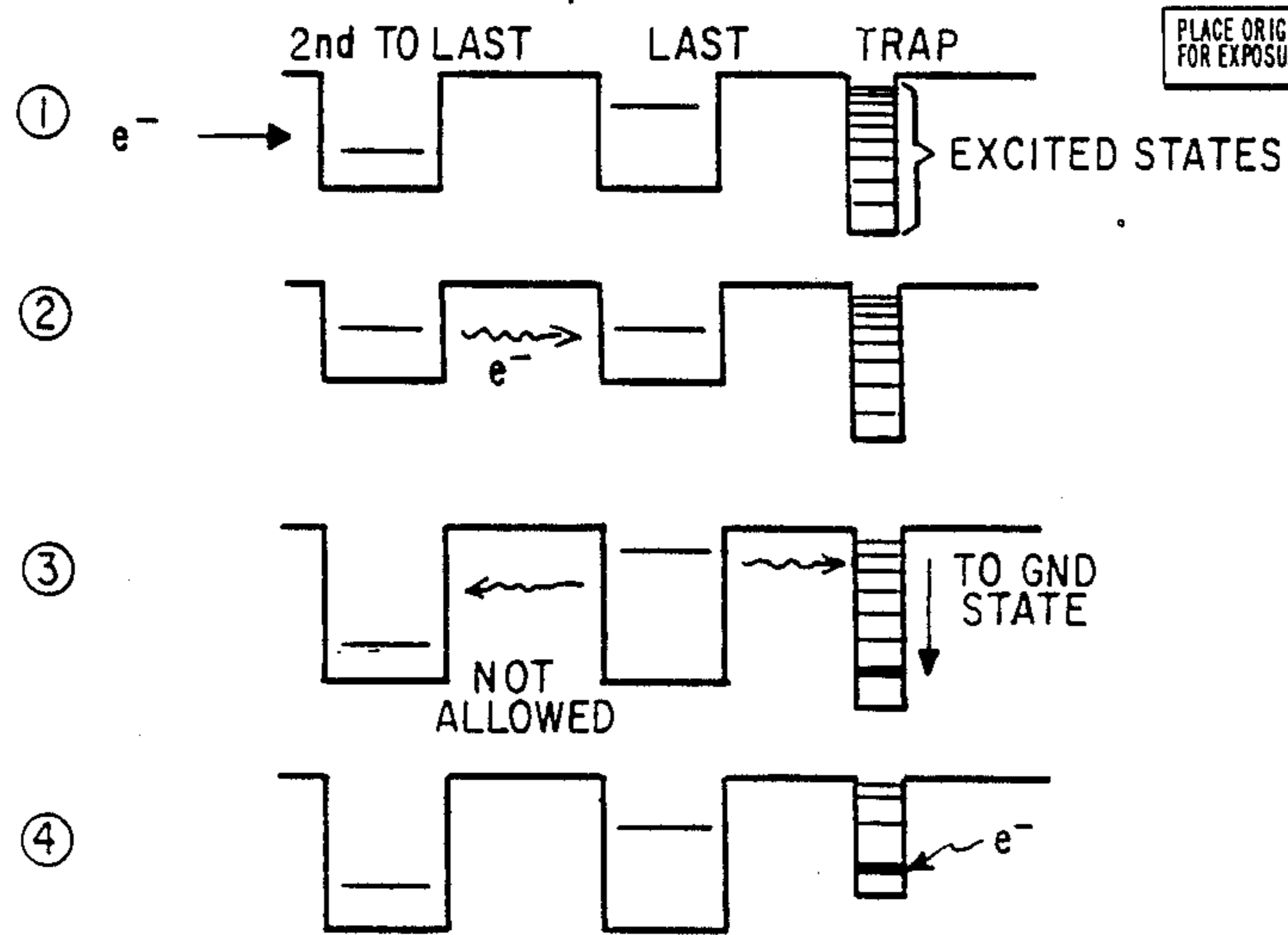
SELF-CONSISTENCY DIAGRAM;
