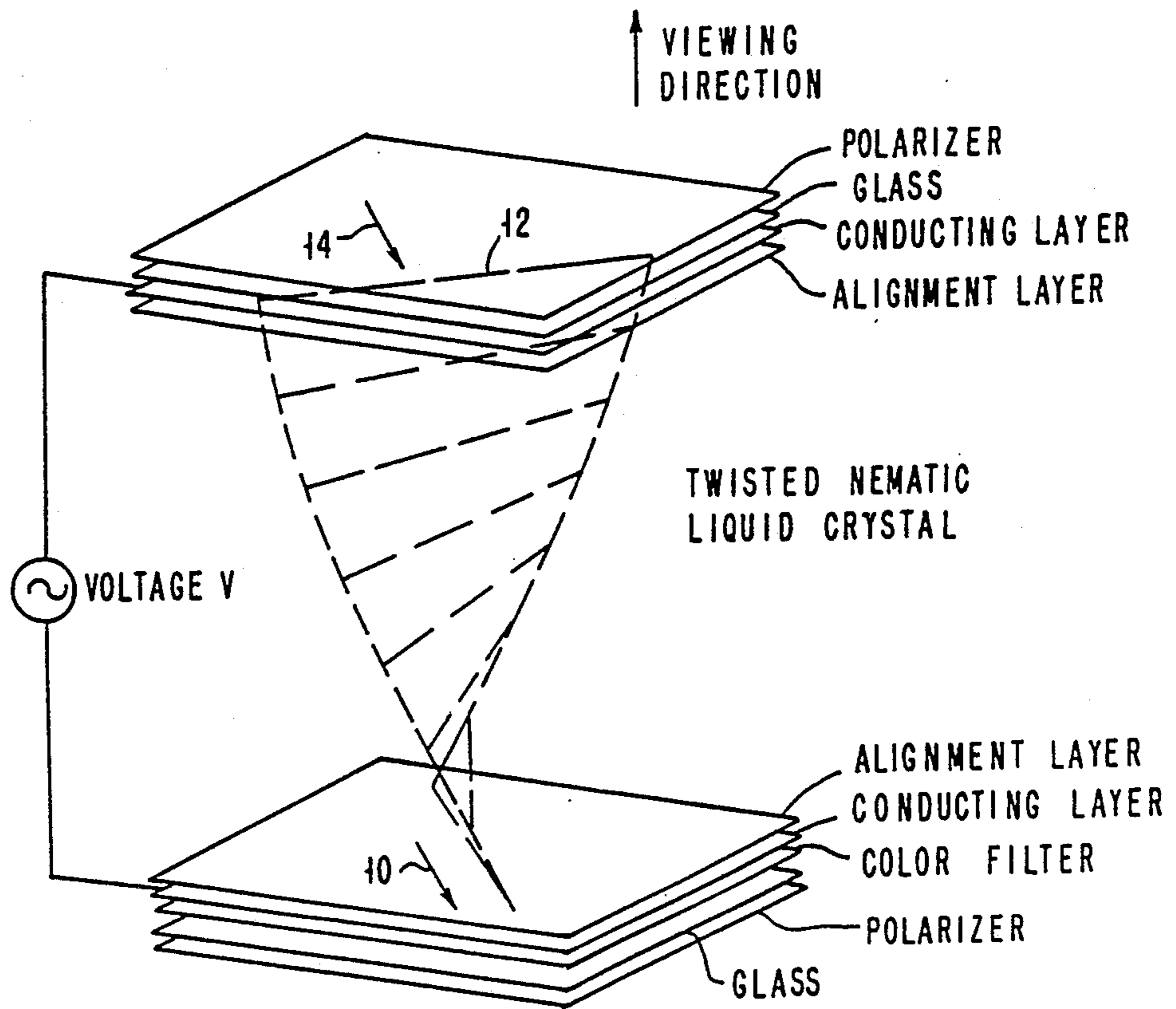
FIG. 1 PRIOR ART 90° TWISTED NEMATIC LCD
