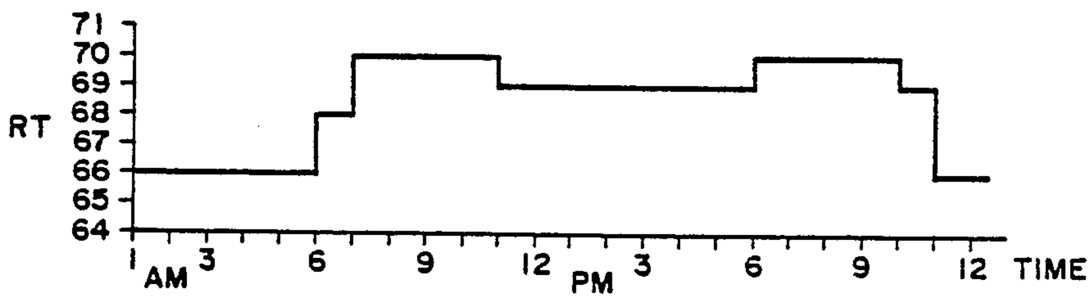
FIGURE 2D HEATING (OCCUPANTS HOME DURING DAY)
