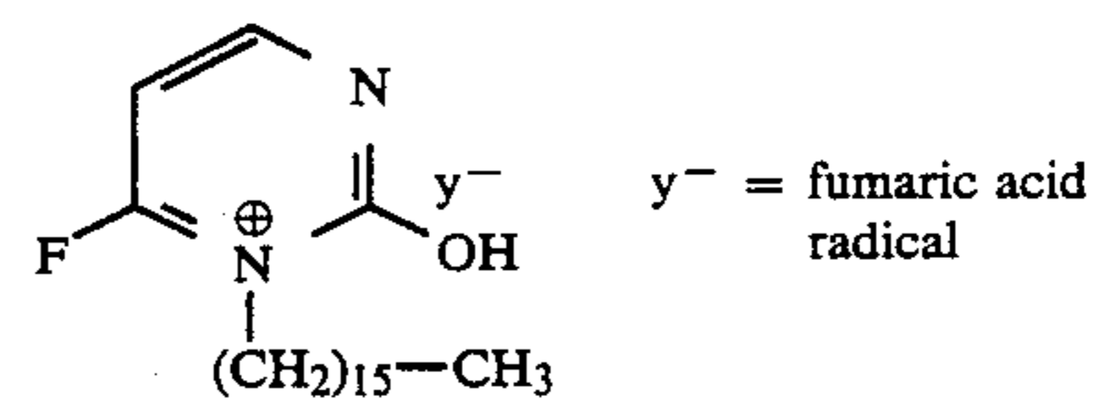
(2-hydroxy-5-fluoro-hexadecylpyrimidinium fumarate)
