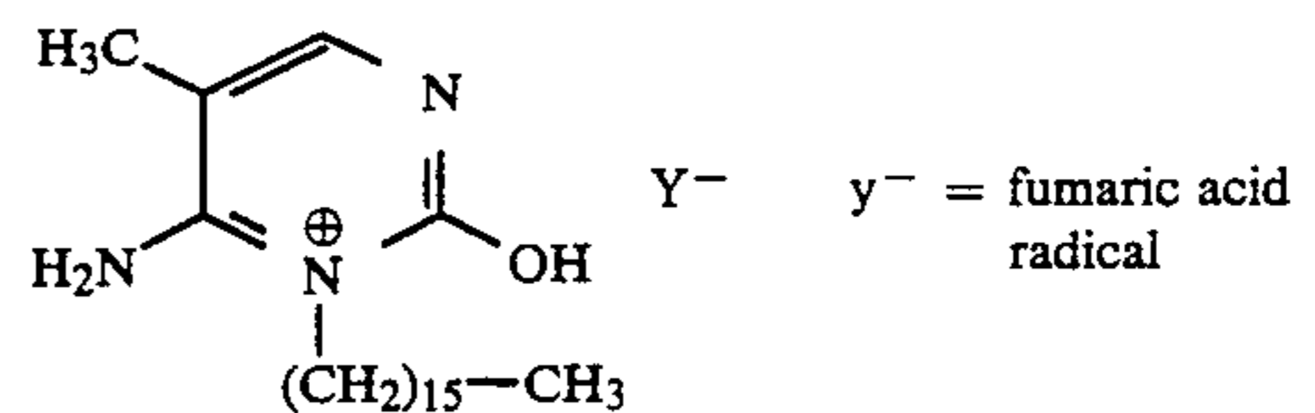
(2-hydroxy-5-methyl-6-amino-hexadecylpyrimidinium fumarate)
