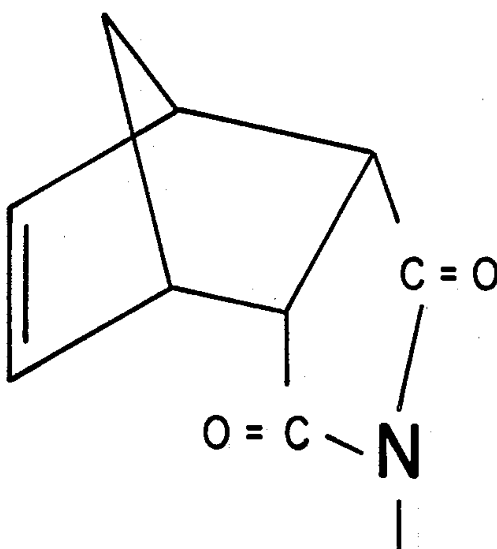
ENDO STEREOISOMER
