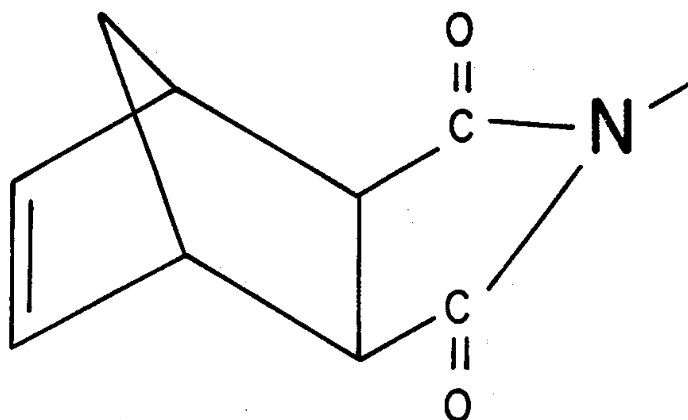
EXO STEREOISOMER
