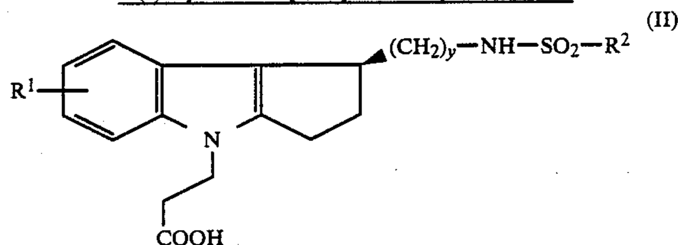
(a) Cycloalkano[1,2-b]indole-sulphonamides
