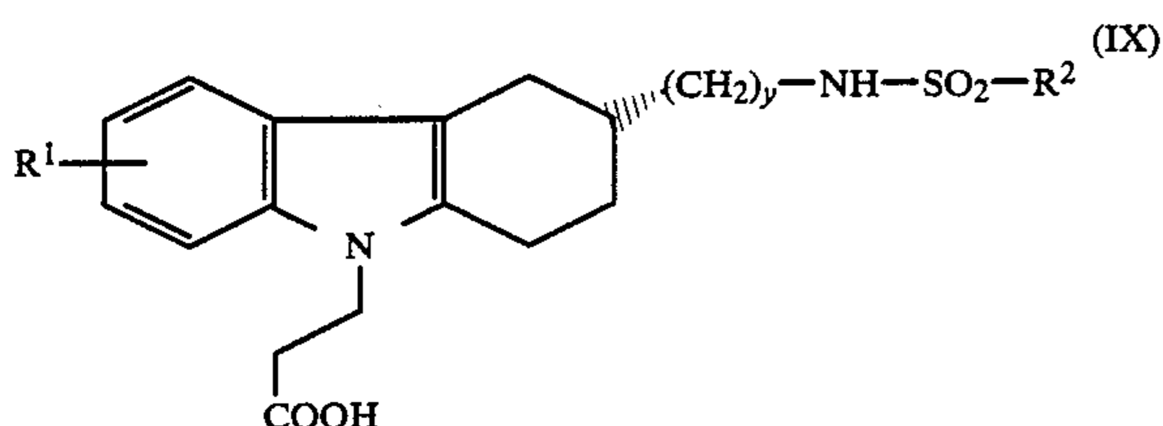
(b) Cycloalkano[1,2-b]indole-sulphonamides
