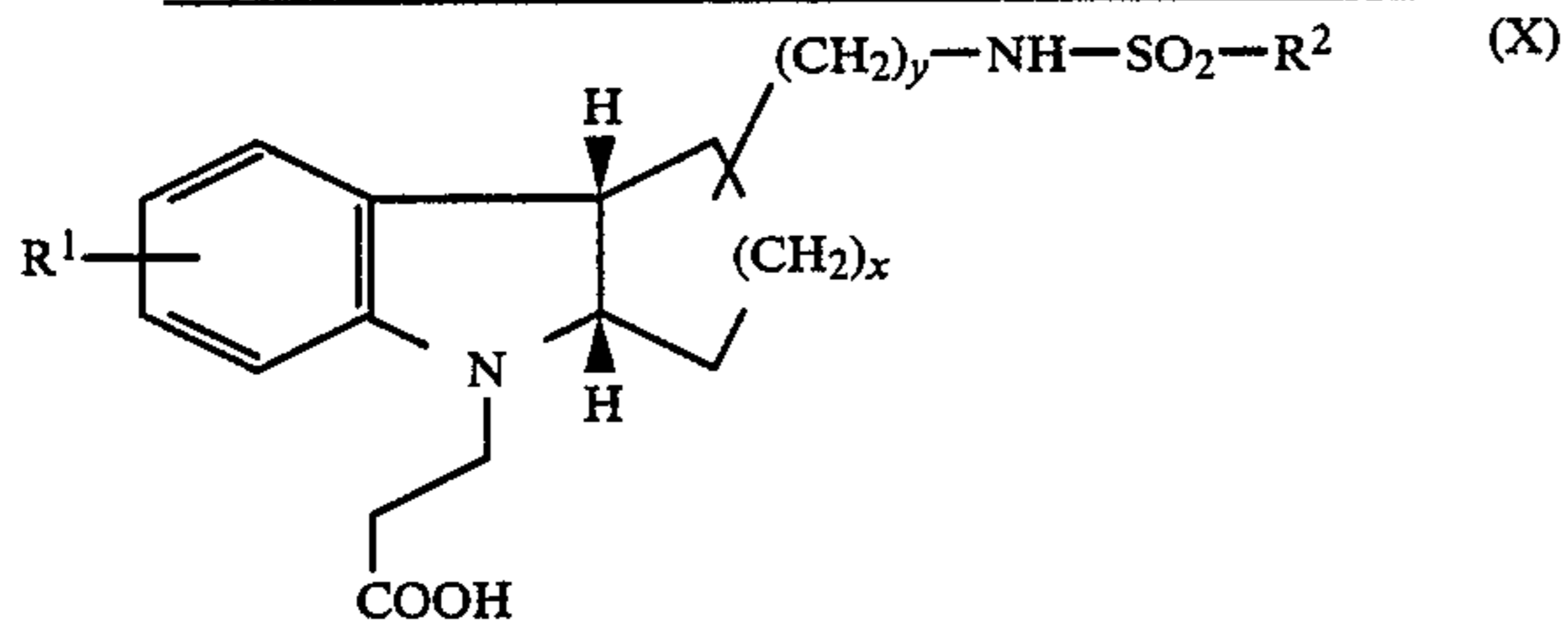
(b) Cycloalkano[1,2-b]indole-sulphonamides
