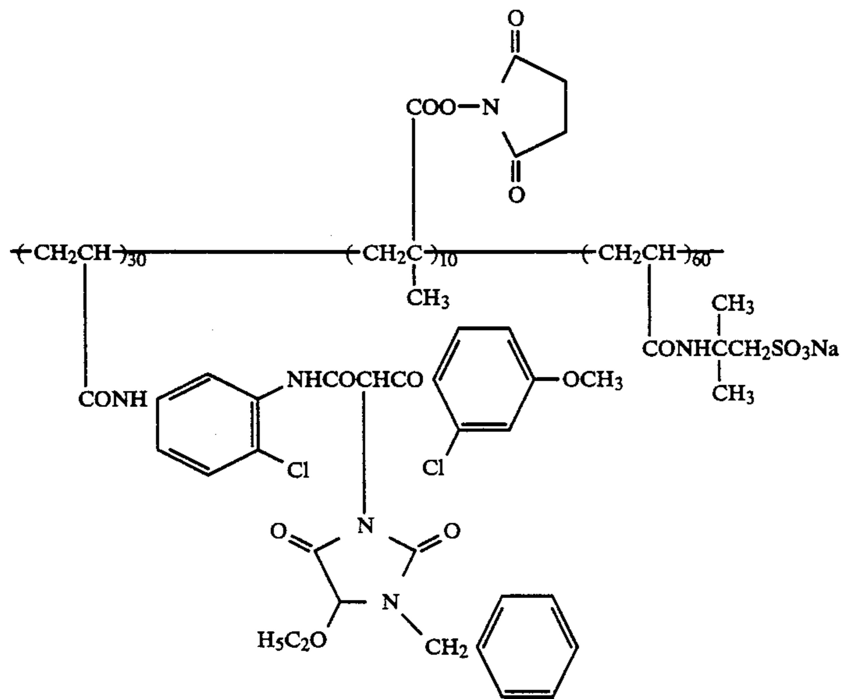
Polymeric Couplers Including the Repeating Unit Represented by Formula (II-A)
