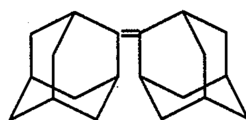
adamantylideneadamantane
