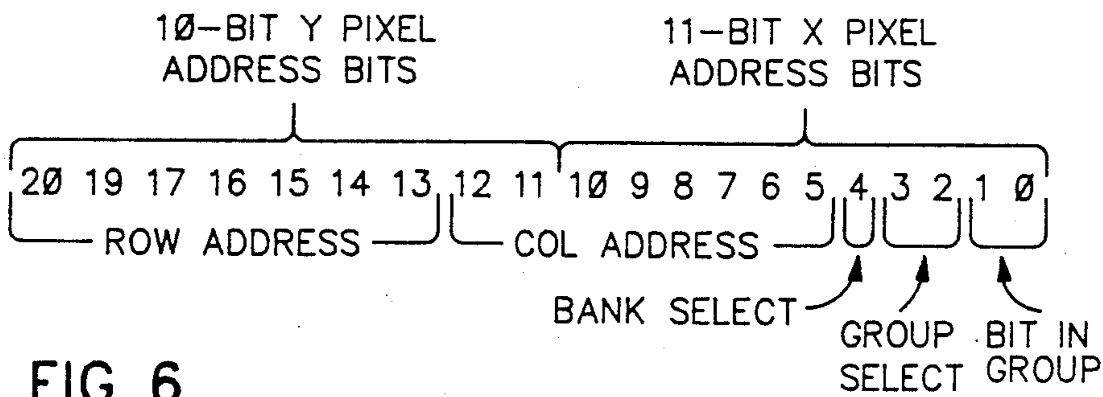
ADDRESSING 16 X 1 TILES
