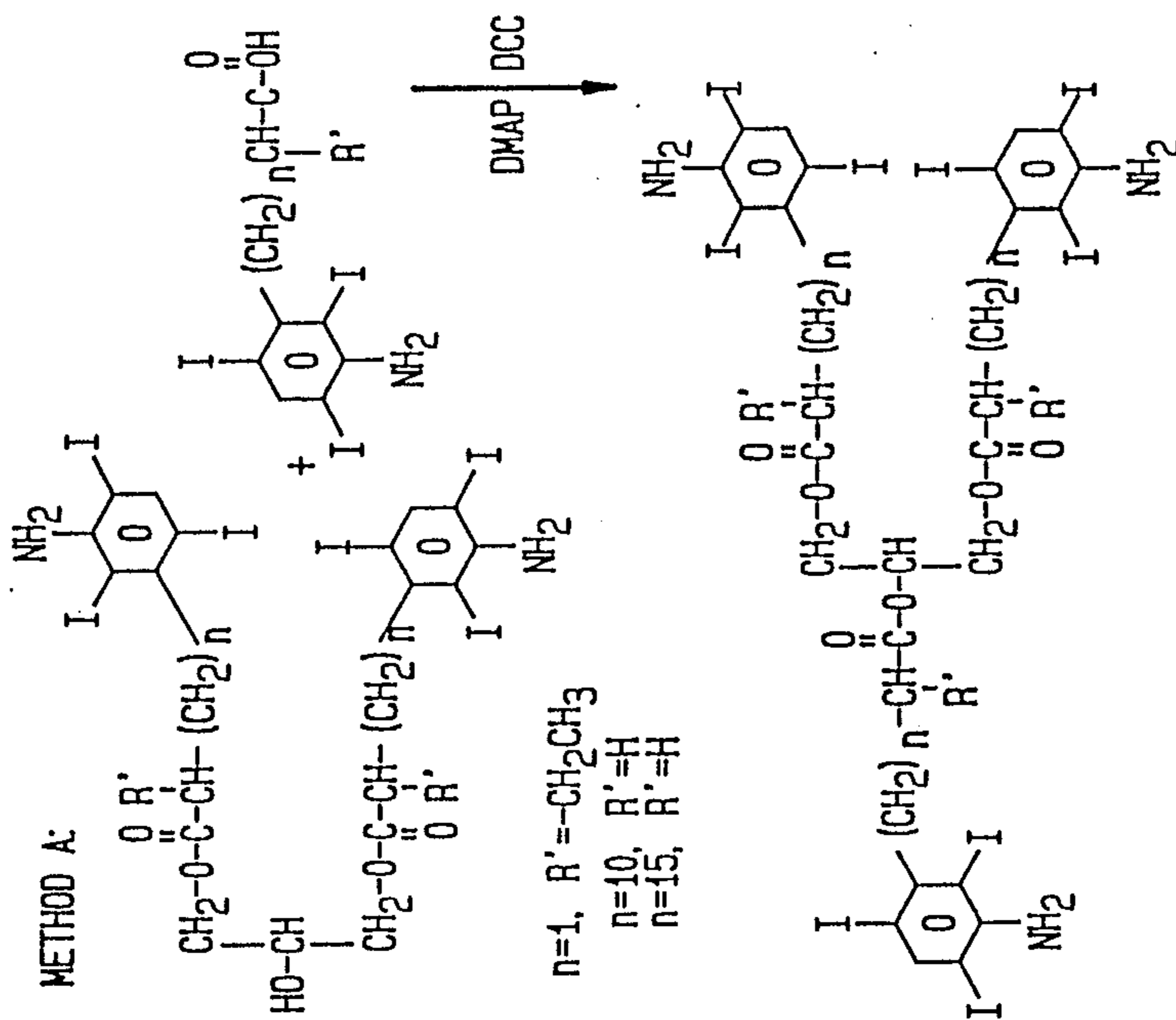
FIG. 4 1, 2, 3-TRISUBSTITUTED TRIGLYCERIDES
