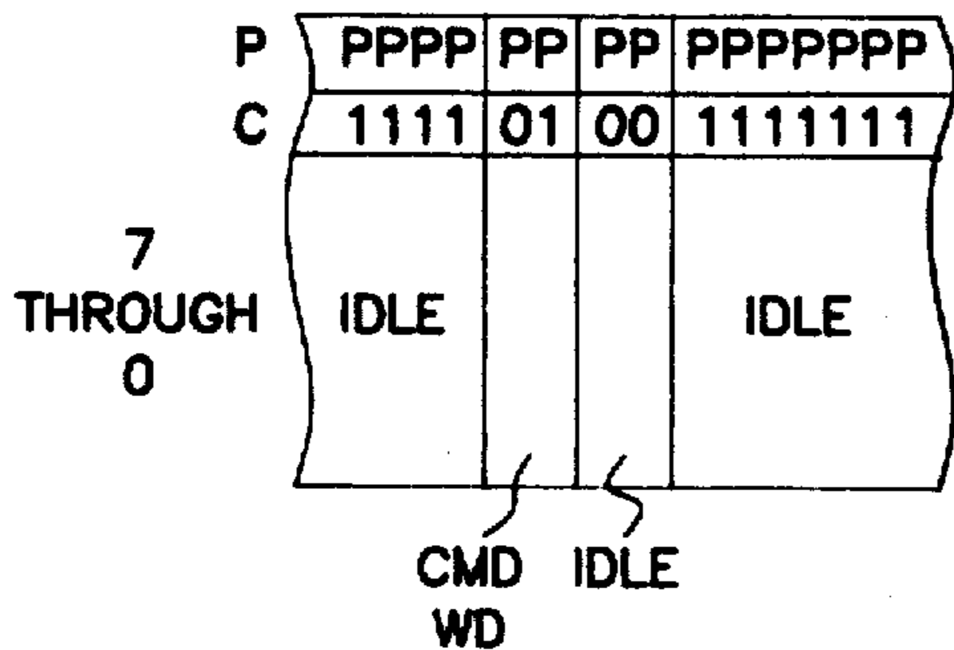
MESSAGE FORMAT (CONTROL / STATUS PRIMARY MESSAGE)
